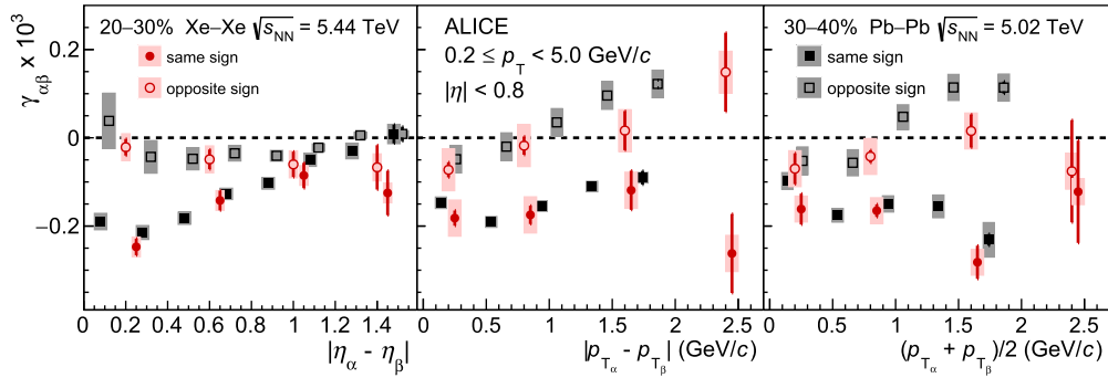
Fig. 2. The dependence of \gamma_{\alpha\beta} on the pseudorapidity difference |\eta_\alpha - \eta_\beta| (left panel), the transverse momentum difference |\rho_{T_\alpha} - \rho_{T_\beta}| (middle panel), and the average transverse momentum (\rho_{T_\alpha} + \rho_{T_\beta})/2 (right panel) for pairs of particles with same (closed markers) and opposite (open markers) charges from 20–30% Xe–Xe collisions at \sqrt{s_{NN}} = 5.44 TeV (red circles) compared to results from 30–40% Pb–Pb collisions at \sqrt{s_{NN}} = 5.02 TeV (black squares) [42]. The Pb–Pb and Xe–Xe same-charge points are slightly shifted along the horizontal axis for better visibility in all panels. Bars (boxes) denote statistical (systematic) uncertainties.
