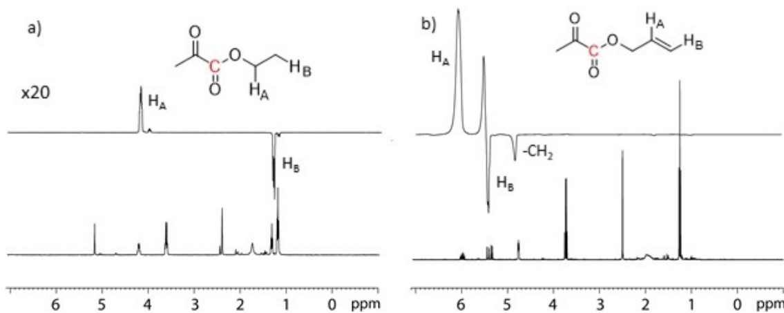
Figure 2. ^1\text{H} -NMR spectra of parahydrogenated ethyl-[1- ^{13}\text{C} ]pyruvate and propargyl-[1- ^{13}\text{C} ]pyruvate obtained in ALTADENA experiments. The proton polarization on the ethyl derivative (a) is considerably lower than on the parahydrogenated propargyl derivative (b).
