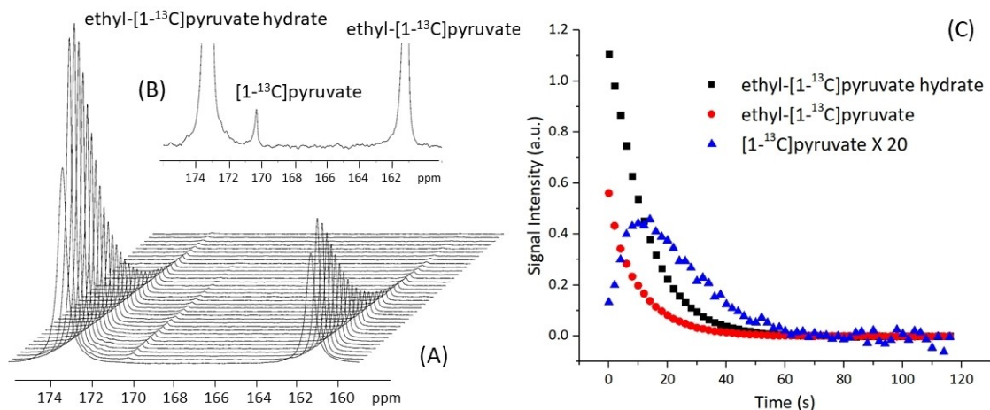
Figure 3. (A) Series of 13 C-NMR spectra acquired upon mixing the pyruvate esterase containing solution (400 U) with the aqueous solution of hyperpolarized ethyl-[1- 13 C]pyruvate. Spectra were acquired using small flip angle pulse (10°) and 2 s delays between successive scans. (B) expanded 13 C-NMR spectrum at maximum intensity of the [1- 13 C]pyruvate signal; (C) Plot of the time dependent changes of the signals of ethyl-[1- 13 C]pyruvate, its hydrated form, and of the [1- 13 C]pyruvate (obtained from the integrals of the peaks in the 13 C-NMR spectra reported in (A)); the [1- 13 C]pyruvate signal intensity is shown multiplied by 20.
