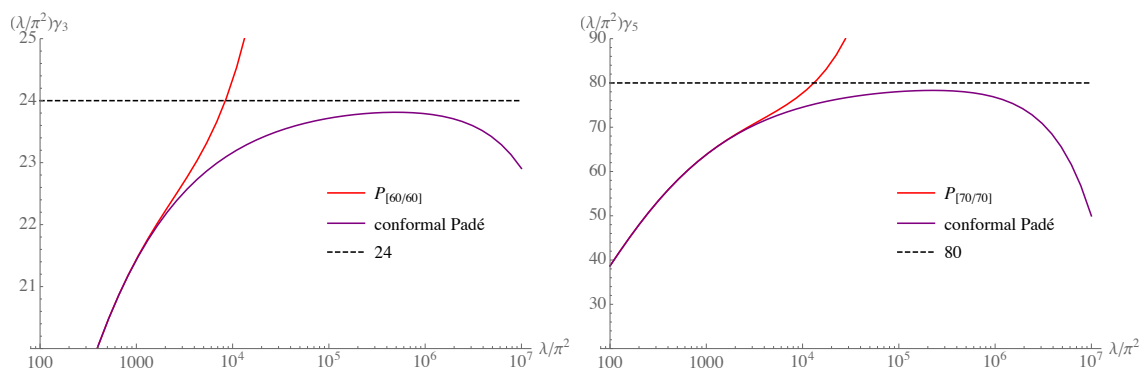
Figure 3. Comparison between the simple and the conformally improved Padé approximants for (\lambda/\pi^2)\gamma_3 (left) and (\lambda/\pi^2)\gamma_5 (right). This quantity is expected to tend to 24 for \gamma_3 and to 80 for \gamma_5 .
