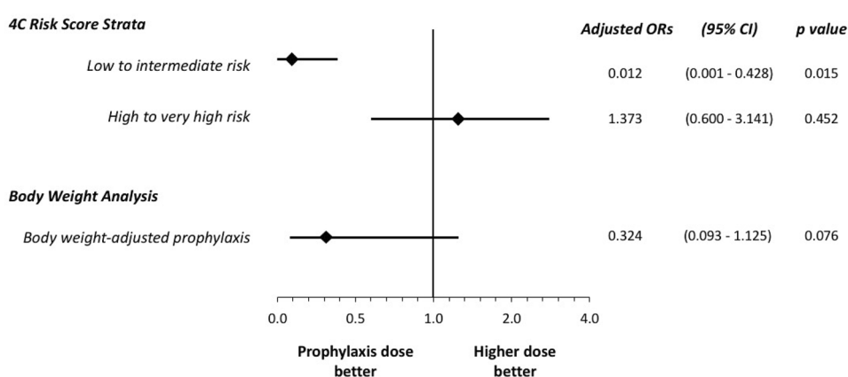
Fig. 3 Adjusted ORs for the primary end-point with: 4000 IU vs. > 4000 IU enoxaparin daily dose in the subgroups with low/intermediate and high/very high risk according to the 4C Mortality Score; ≤ 70 IU/Kg vs. > 70 IU/Kg enoxaparin daily regimen. CI Confidence interval; OR Odds ratio
