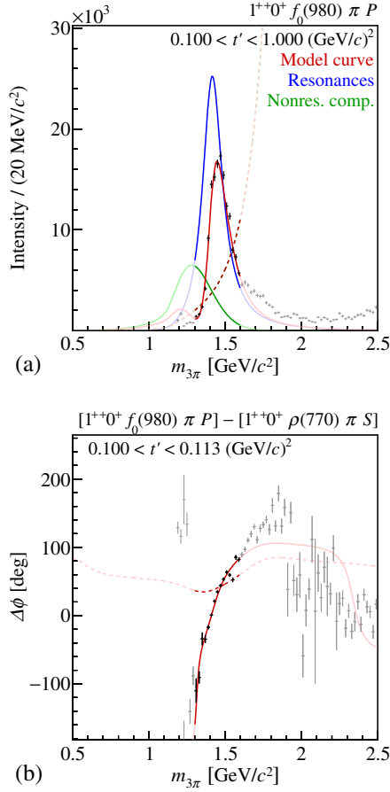
FIG. 36. (a) t' -summed intensity of the 1^{++}0^+ f_0(980)\pi P wave and (b) phase of this wave with respect to the 1^{++}0^+ \rho(770)\pi S wave in the lowest t' bin. The result of the main fit is represented by the continuous curves. The fit, in which the a_1(1420) component was removed from the model, is represented by the dashed curves. These curves correspond to the nonresonant component. The model and the wave components are represented as in Fig. 28.
