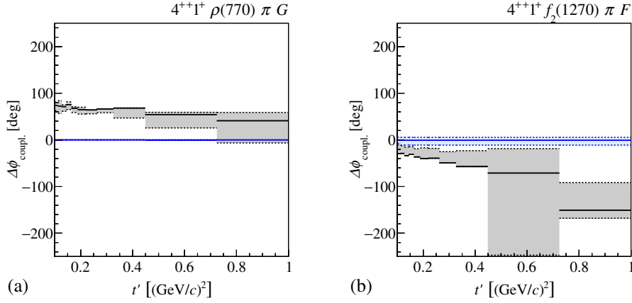
FIG. 55. Similar to Fig. 50 but for the wave components in (a) the 4^{++}1^+\rho(770)\pi G and (b) the 4^{++}1^+f_2(1270)\pi F wave. The coupling phases of the a_4(2040) (blue lines) and the nonresonant component (black lines) are shown relative to the a_4(2040) in the 4^{++}1^+\rho(770)\pi G wave.
