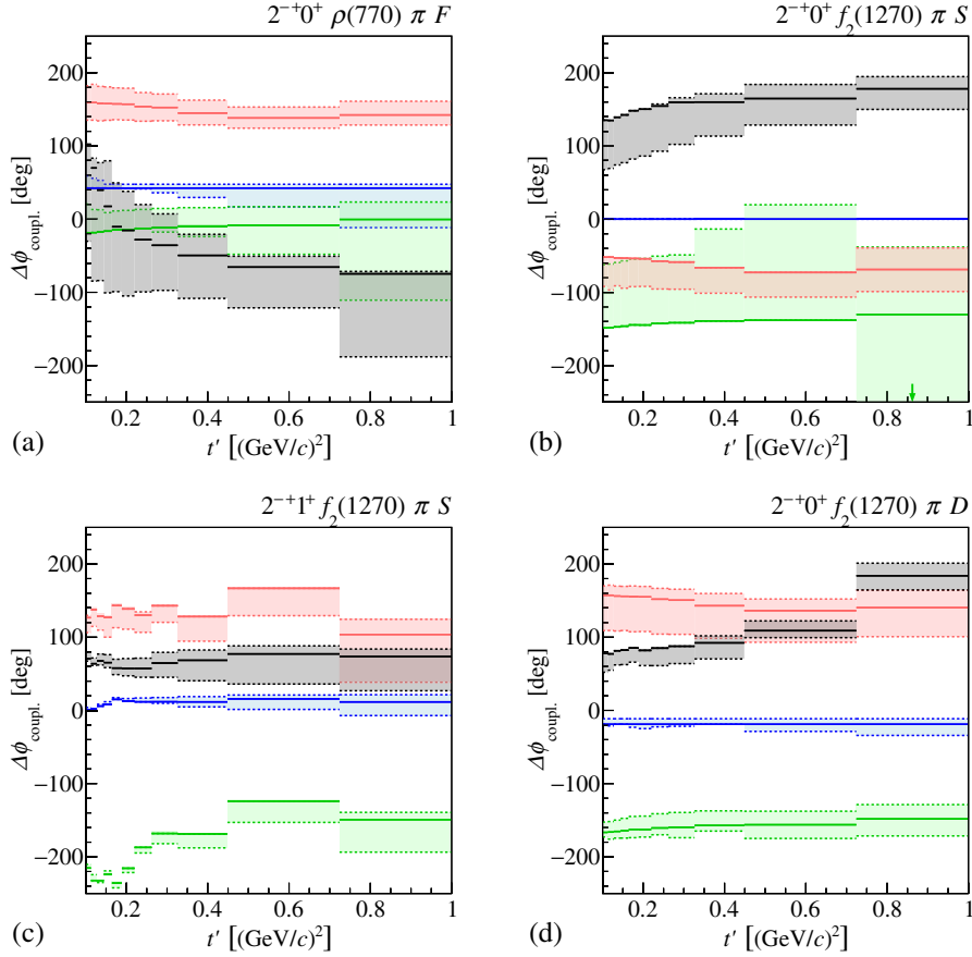
FIG. 50. t' dependence of the coupling phases of the wave components in (a) the 2^{-+}0^{+}\rho(770)\pi F , (b) the 2^{-+}0^{+}f_2(1270)\pi S , (c) the 2^{-+}1^{+}f_2(1270)\pi S , and (d) the 2^{-+}0^{+}f_2(1270)\pi D wave. The coupling phases of the \pi_2(1670) (blue lines), the \pi_2(1880) (green lines), the \pi_2(2005) (red lines), and the nonresonant components (black lines) are shown relative to the \pi_2(1670) in the 2^{-+}0^{+}f_2(1270)\pi S wave. For each wave component, the magnitude of the effects observed in the systematic studies (see Sec. V) is illustrated qualitatively by two sets of dashed lines with shaded area in between (see text).
