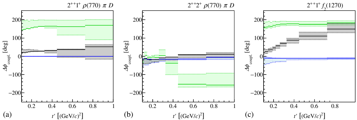
FIG. 54. Similar to Fig. 50 but for the wave components in (a) the 2^{++}1^+\rho(770)\pi D , (b) the 2^{++}2^+\rho(770)\pi D , and (c) the 2^{++}1^+f_2(1270)\pi P wave. The coupling phases of the a_2(1320) (blue lines), the a_2(1700) (green lines), and the nonresonant component (black lines) are shown relative to the a_2(1320) in the 2^{++}1^+\rho(770)\pi D wave.
