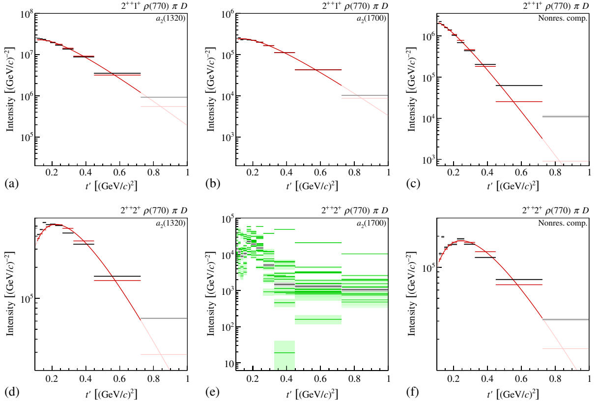
FIG. 17. Similar to Fig. 7 but showing the t' spectra of the components in the 2^{++}\rho(770)\pi D waves with (upper row) M^e = 1^+ and (lower row) M^e = 2^+ as given by Eq. (40): (left) a_2(1320) component, (center) a_2(1700) component, and (right) nonresonant components. The red curves and horizontal lines represent fits using Eq. (41). (e) shows in addition to the a_2(1700) t' spectrum from the main fit (black/gray) the t' spectra obtained in the various systematic studies (central values shown in green, statistical uncertainties in light green).
