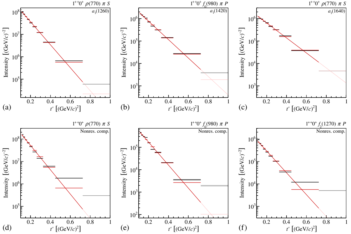
FIG. 33. Similar to Fig. 7, but showing the t' spectra of some of the components in the three 1^{++} waves as given by Eq. (40). The red curves and horizontal lines represent fits using Eq. (41).
