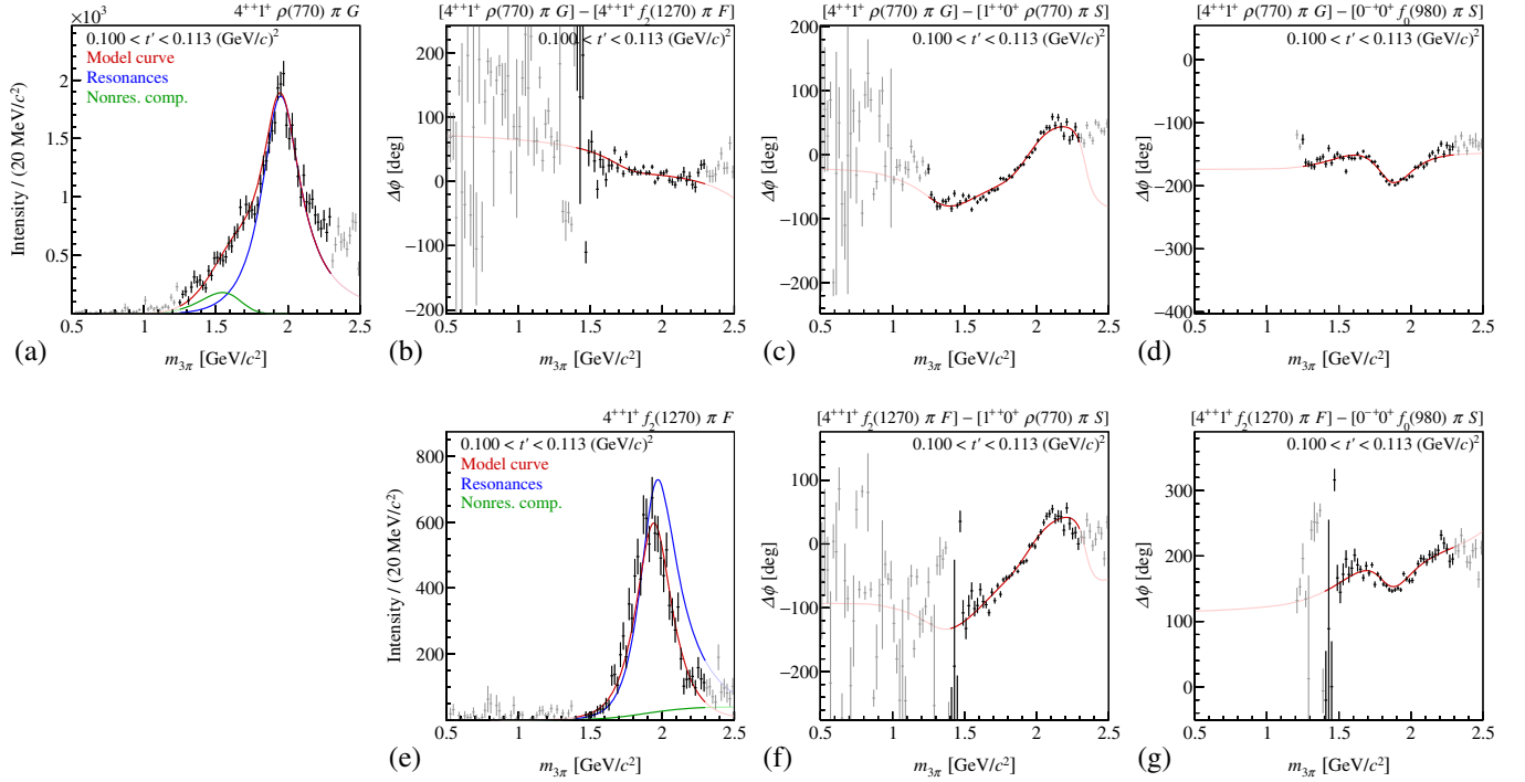
FIG. 12. Amplitudes of the two J^{PC} = 4^{++} waves in the lowest t' bin. (a) through (d): intensity distribution and relative phases for the 4^{++}1^+\rho(770)\pi G wave. (e) through (g): intensity distribution and relative phases for the 4^{++}1^+f_2(1270)\pi F wave. The model and the wave components are represented as in Fig. 10, except that here the blue curve represents the a_4(2040) .
