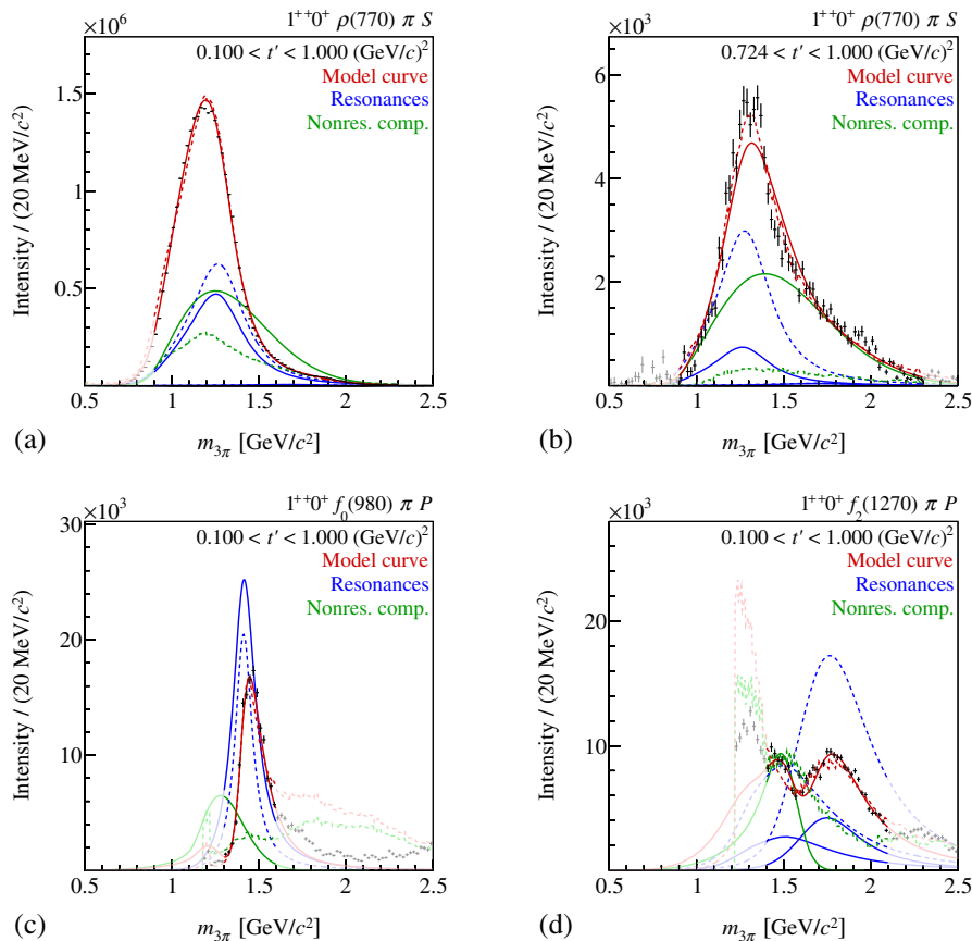
FIG. 35. (a) t' -summed intensity of the 1^{++}0^+\rho(770)\pi S wave. (b) Intensity of this wave in the highest t' bin. (c) and (d): The t' -summed intensity of the 1^{++}0^+f_0(980)\pi P and the 1^{++}0^+f_2(1270)\pi P wave, respectively. The result of the main fit is represented by the continuous curves. The fit, in which the parametrization of the nonresonant amplitude was replaced by the square root of the intensity distribution of the partial-wave decomposition of Deck Monte Carlo data [Study (N); see Sec. V], is represented by the dashed curves. The model and the wave components are represented as in Fig. 28.
