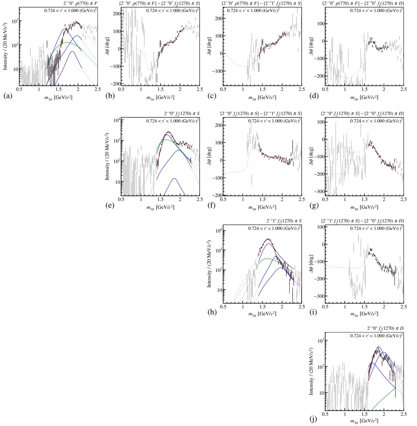
FIG. 23. Similar to Fig. 22 but for the highest t' bin.
