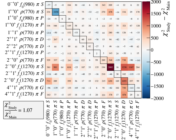
FIG. 26. Similar to Fig. 9, but for the study in which the \pi_2(2005) resonance was omitted from the fit model.
