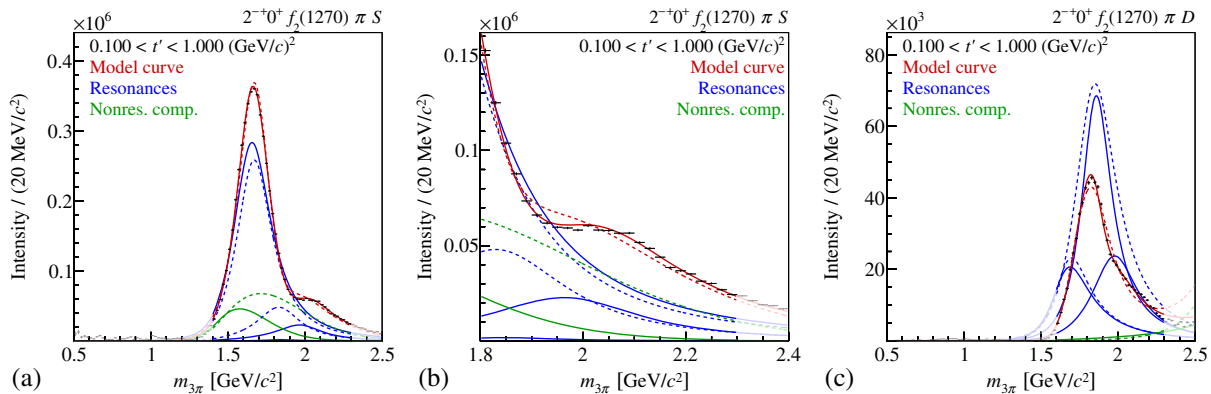
FIG. 27. t' -summed intensities of (a) the 2^{-+0^+} f_2(1270) \pi S wave and (c) the 2^{-+0^+} f_2(1270) \pi D wave with the result of the main fit (continuous curves) and of the fit in which the \pi_2(2005) resonance was omitted from the fit model (dashed curves). The model and the wave components are represented as in Fig. 21. In (b), a zoomed view of the high-mass region in (a) is shown.
