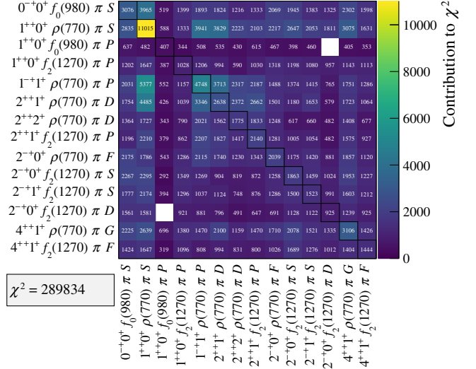
FIG. 6. Contributions from the intensities and interference terms to the \chi^2 in Eq. (34) summed over the m_{3\pi} and l' bins. The two cells for the interference term of the 1^{++}0^+f_0(980)\pi P and 2^{-+}0^+f_2(1270)\pi D waves are empty because the fit ranges for these two waves do not overlap (see Table II).
