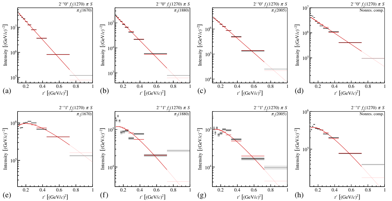
FIG. 24. Similar to Fig. 7, but showing the t' spectra of the components in the two 2^{-+}f_2(1270)\pi S waves as given by Eq. (40): (top row) M^e = 0^+ wave and (bottom row) M^e = 1^+ wave; (first column) \pi_2(1670) component, (second column) \pi_2(1880) component, (third column) \pi_2(2005) component, and (fourth column) nonresonant components. The red curves and horizontal lines represent fits using Eq. (41).
