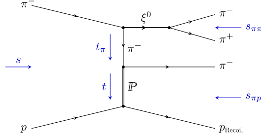
FIG. 8. Example for a nonresonant production process for the 3\pi final state as proposed by Deck [44]. In this process, the beam pion dissociates into the isobar \xi^0 and the bachelor \pi^- , followed by diffractive scattering of one of these beam fragments (typically the \pi^- , as shown here) off the target proton.
