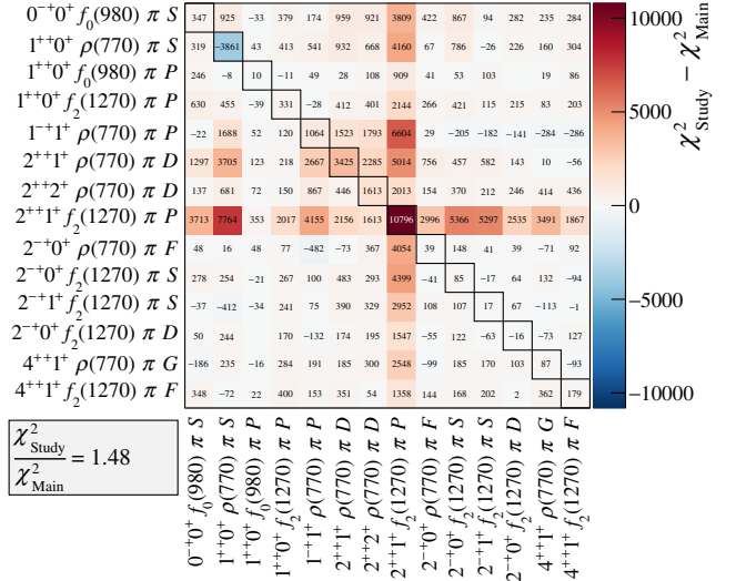
FIG. 19. Similar to Fig. 9, but for the study, in which the a_2(1700) component was omitted from the fit model.
