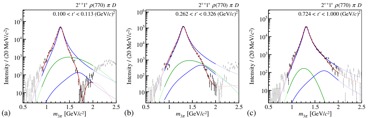
FIG. 16. Intensity distributions of the 2^{++}1^+\rho(770)\pi D wave for three t' bins shown in logarithmic scale. The model and the wave components are represented as in Fig. 14.
