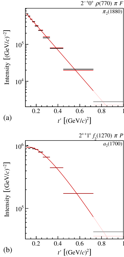
FIG. 7. Examples for t' spectra of wave components extracted according to Eq. (40). The black horizontal lines indicate the central values, and the gray boxes the statistical uncertainties (see text for details). (a) \pi_2(1880) component in the 2^{-+}0^+\rho(770)\pi F wave; (b) a_2(1700) component in the 2^{++}1^+f_2(1270)\pi P wave. The red curves and lines show the result of a fit of Eq. (41) to the data (see text for details).
