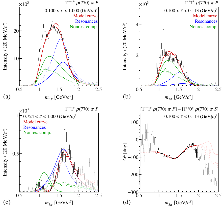
FIG. 46. (a) t' -summed intensity of the 1^{-+}1^+\rho(770)\pi P wave. (b) and (c): Intensity of this wave in the lowest and highest t' bins, respectively. (d) Phase of the 1^{-+} wave relative to the 1^{++0^+}\rho(770)\pi S wave in the lowest t' bin. The result of the main fit is represented by the continuous curves. The fit, in which the parametrization of the nonresonant amplitude was replaced by the square root of the intensity distribution of the partial-wave decomposition of Deck Monte Carlo data [Study (N); see Sec. V], is represented by the dashed curves. The model and the wave components are represented as in Fig. 43.
