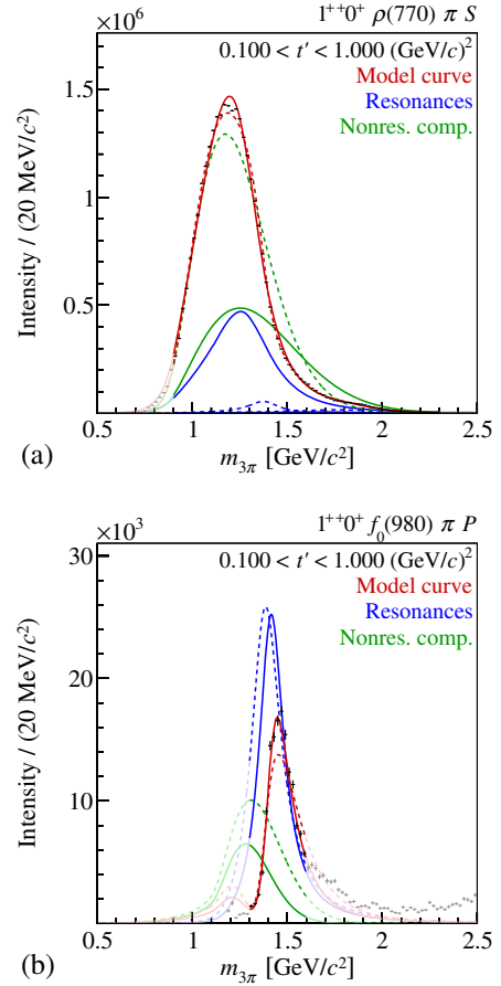
FIG. 38. t' -summed intensities of the 1^{++}0^+ \rho(770)\pi S and the 1^{++}0^+ f_0(980)\pi P wave. The result of the main fit is represented by the continuous curves. The fit, in which the a_1(1420) resonance in the 1^{++}0^+ f_0(980)\pi P wave was replaced by the a_1(1260) , is represented by the dashed curves. The model and the wave components are represented as in Fig. 28.
