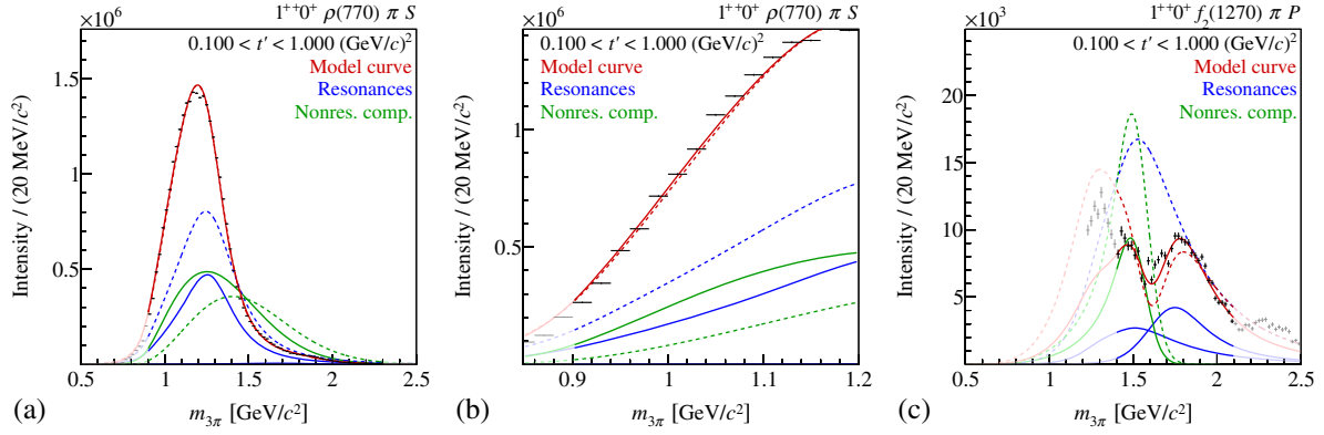
FIG. 42. t' -summed intensities of (a) the 1^{++}0^+\rho(770)\pi S wave and (c) the 1^{++}0^+f_2(1270)\pi P wave. In (b), a zoomed view of (a) is shown. The result of the main fit is represented by the continuous curves. The fit, in which the a_1(1640) component was removed from the fit model, is represented by the dashed curves. The model and the wave components are represented as in Fig. 28.
