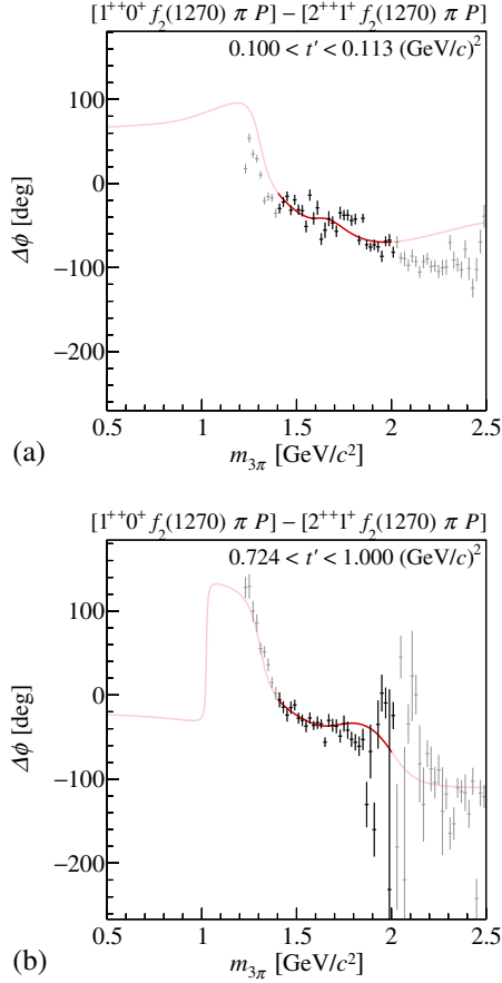
FIG. 32. Phase of the 1^{++}0^+ f_2(1270)\pi P wave relative to the 2^{++}1^+ f_2(1270)\pi P wave, (a) for the lowest t' bin and (b) for the highest t' bin. The model is represented as in Fig. 28.
