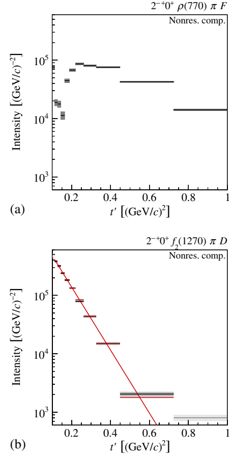
FIG. 25. Similar to Fig. 7, but showing the t' spectra of the nonresonant components (a) in the 2^{-+}0^{+}\rho(770)\pi F wave and (b) in the 2^{-+}0^{+}f_2(1270)\pi D wave. The red curve and horizontal lines in (b) represent a fit using Eq. (41).
