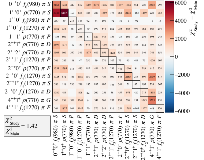
FIG. 9. Decomposition of the \chi^2 difference between the main fit and the fit, in which the parametrization of the nonresonant amplitude was replaced by the square root of the intensity distribution of the partial-wave projections of Deck Monte Carlo data [Study (N)]. The \chi^2 difference is visualized in the form of a matrix, which shows the contributions (summed over the m_{3\pi} and t' bins) from the intensities and interference terms to the \chi^2 difference. Positive values (red colors) indicate that the data are described less well in the study. The rare negative values (blue colors) indicate that the data are described better in the study.
