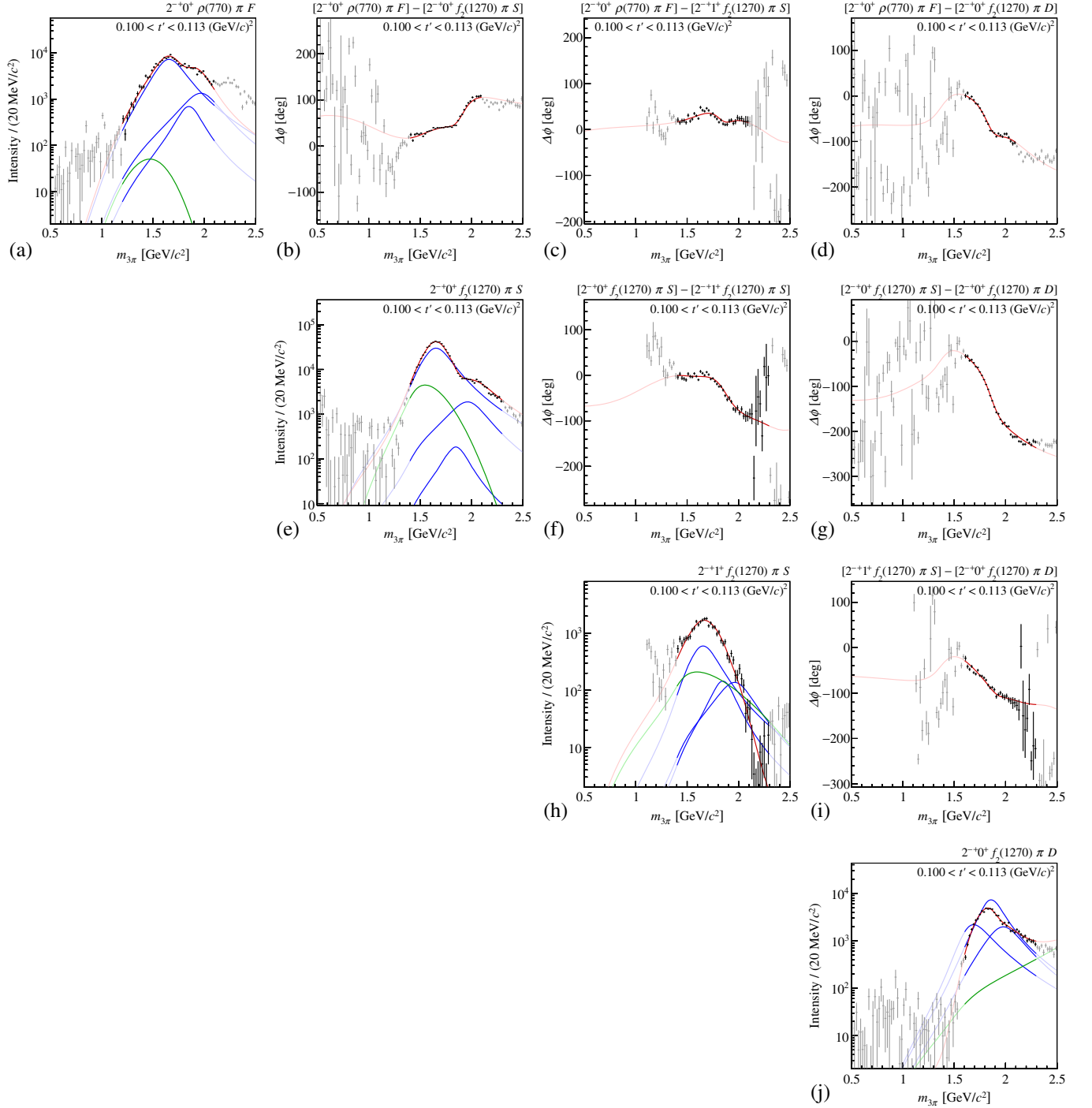
FIG. 22. Amplitudes of the four J^{PC} = 2^{-+} waves in the lowest t' bin. (a) through (d): Intensity distribution and relative phases for the 2^{-+}0^+\rho(770)\pi F wave. (e) through (g): Intensity distribution and relative phases for the 2^{-+}0^+f_2(1270)\pi S wave. (h) and (i): Intensity distribution and relative phase for the 2^{-+}1^+f_2(1270)\pi S wave. (j): Intensity distribution for the 2^{-+}0^+f_2(1270)\pi D wave. The model and the wave components are represented as in Fig. 21.
