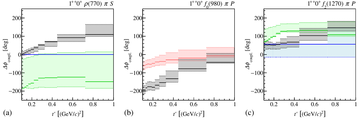
FIG. 53. Similar to Fig. 50 but for the wave components in (a) the 1^{++}0^+\rho(770)\pi S , (b) the 1^{++}0^+f_0(980)\pi P , and (c) the 1^{++}0^+f_2(1270)\pi P wave. The coupling phases of the a_1(1260) (blue lines), the a_1(1420) (red lines), the a_1(1640) (green lines), and the nonresonant components (black lines) are shown relative to the a_1(1260) in the 1^{++}0^+\rho(770)\pi S wave.
