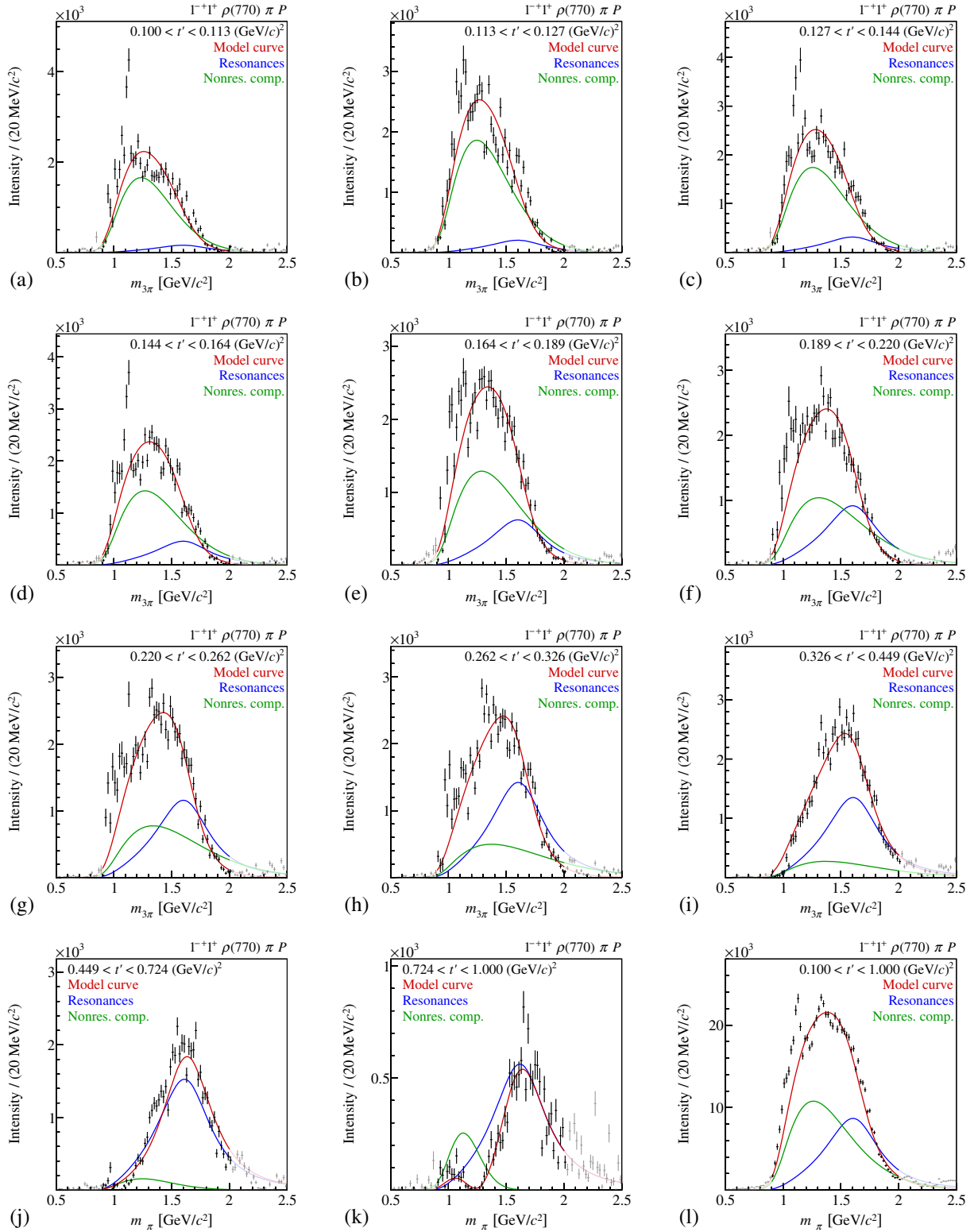
FIG. 43. (a) to (k): Intensity distribution of the 1^{--}1^{+}\rho(770)\pi P wave in the 11 t' bins. (l) The t' -summed intensity. The model and the wave components are represented as in Fig. 10, except that the blue curve represents the \pi_1(1600) .
