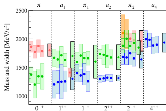
FIG. 1. Masses and widths of light isovector mesons with positive C parity and a 3\pi decay mode. For each resonance, the four most recent measurements of masses (circles) and widths (vertical size of boxes), as listed by the PDG [10], are compared to the masses and widths obtained in this analysis (crosses and black-framed boxes, respectively). The measurements are grouped according to the J^{PC} quantum numbers of the states. Higher excitations with the same J^{PC} are shown in different colors.
