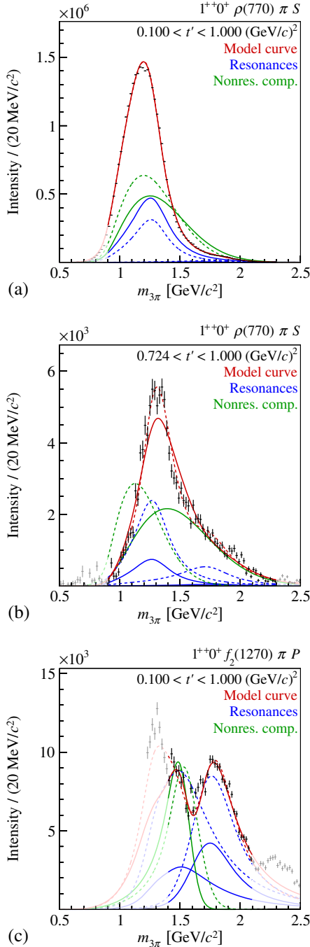
FIG. 34. (a) t' -summed intensity of the 1^{++}0^+\rho(770)\pi S wave. (b) intensity of this wave in the highest t' bin. (c) t' -summed intensity of the 1^{++}0^+f_2(1270)\pi P wave. The result of the main fit is represented by the continuous curves. The fit, in which none of the coupling amplitudes of the resonance components was constrained via Eq. (21) [Study (M); see Sec. V], is represented by the dashed curves. The model and the wave components are represented as in Fig. 28.
