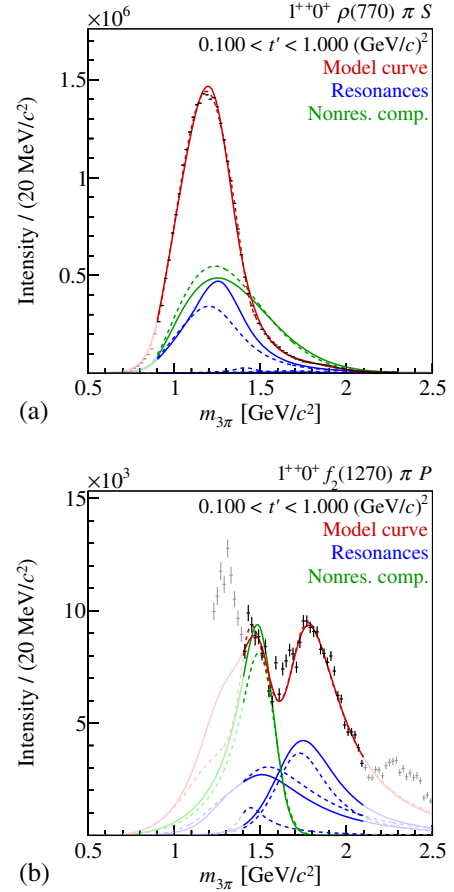
FIG. 40. t' -summed intensities of (a) the 1^{++}0^{+}\rho(770)\pi S wave and (b) the 1^{++}0^{+}f_2(1270)\pi P wave. The result of the main fit is represented by the continuous curves. The fit, in which the a_1(1420) resonance is also included in the 1^{++}0^{+}\rho(770)\pi S and 1^{++}0^{+}f_2(1270)\pi P waves, is represented by the dashed curves. The model and the wave components are represented as in Fig. 28.
