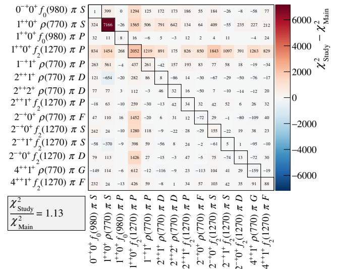
FIG. 41. Similar to Fig. 9, but for the study, in which the a_1(1640) resonance was omitted from the fit model.
