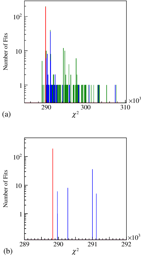
FIG. 5. (a) Distribution of the \chi^2 values of the 832 fits that converged out of the 1000 fit attempts. The selected physical solution (see text) is shown in red. Additional solutions that are considered physical are shown in blue and unphysical solutions in green. (b) Corresponding distribution after removing all unphysical solutions. Note the narrower \chi^2 range.
