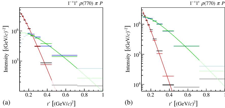
FIG. 45. Similar to Fig. 11, but showing the t' spectra of the two J^{PC} = 1^{-+} wave components as given by Eq. (40): the \pi_1(1600) component is shown as blue lines and light blue boxes, and the nonresonant component as black lines and gray boxes. The red and green curves and horizontal lines represent fits using Eq. (41). (a) The result of the main fit. (b) The result of a fit, in which the parametrization of the nonresonant amplitude was replaced by the square root of the intensity distribution of the partial-wave decomposition of Deck Monte Carlo data [Study (N); see Sec. V and Fig. 46].
