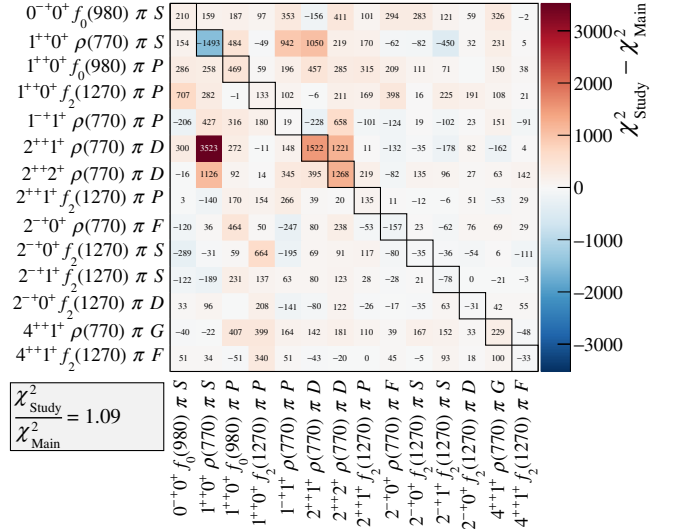
FIG. 37. Similar to Fig. 9, but for the study, in which the a_1(1420) resonance in the 1^{++}0^+ f_0(980)\pi P wave was replaced by the a_1(1260) .
