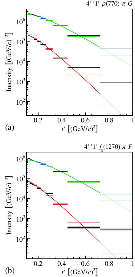
FIG. 13. Similar to Fig. 11, but showing the t' spectra of (a) the 4^{++}1^+\rho(770)\pi G and (b) the 4^{++}1^+f_2(1270)\pi F wave components as given by Eq. (40): the a_4(2040) component is shown as blue lines and light blue boxes, and the nonresonant components as black lines and gray boxes. The red and green curves and horizontal lines represent fits using Eq. (41).
