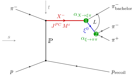
FIG. 2. Diffractive dissociation of a beam pion on a target proton into the \pi^- \pi^- \pi^+ final state via an intermediate 3\pi state X^- . The decay of X^- is described using the isobar model, which assumes that the decay proceeds via an intermediate \pi^- \pi^+ state \xi^0 , the so-called isobar. At the two decay vertices, the couplings \alpha_{X^- \rightarrow \xi^0 \pi} (vertex 1) and \alpha_{\xi^0 \rightarrow \pi^- \pi^+} (vertex 2) appear, which are in general complex numbers.
