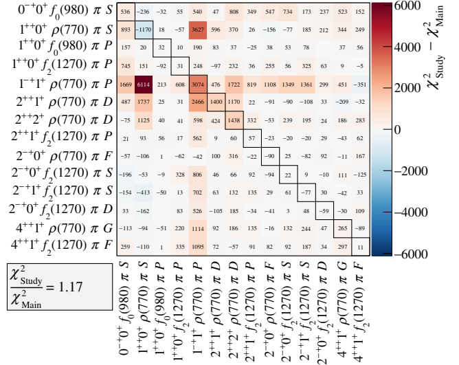
FIG. 47. Similar to Fig. 9, but for the study, in which the \pi_1(1600) resonance was omitted from the fit model.
