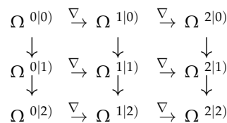
Figure 1. The pseudoform complexes.
