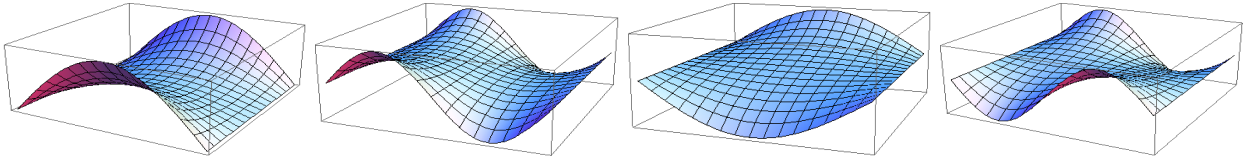
FIGURE 3. Qualitative behavior of some eigenfunctions of (32).
