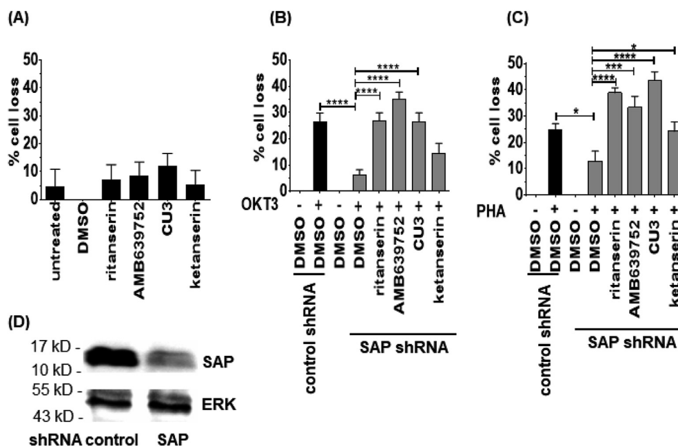
Fig. 8. DGK \alpha inhibitors rescues RICD in SAP deficient Jurkat cells. Jurkat T cells (control shRNA \blacksquare and SAP shRNA \square ) were treated with ritanserin, AMB639752, CU-3 or ketanserin (1 \mu M) and plated on a 96 well flat bottom plate previously coated with nothing (A), anti CD3 (OKT3 50 \mu g/ml, B) and PHA (50 \mu g/ml, C). After 24 h of incubation, live cells were counted using the trypan blue exclusion assay and expressed as % of cell loss respect to untreated controls. The data are the means of \pm SEM of at least five experiments performed in triplicate. D) Western blot confirming the silencing of SAP in SAP shRNA Jurkat cells compared with control shRNA Jurkat cells.
