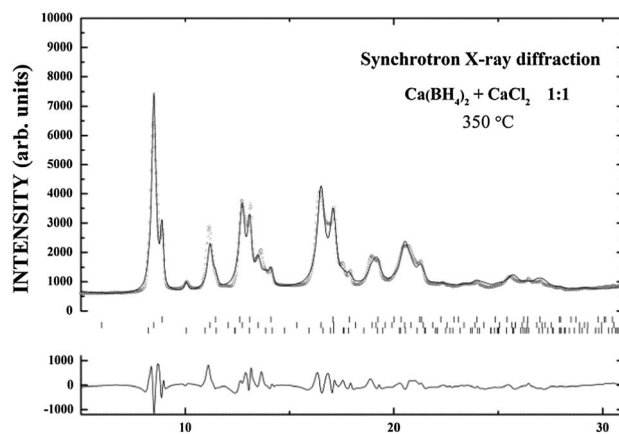
Fig. 2 Rietveld refinement for SR-PXD data of ball milled \text{Ca}(\text{BH}_4)_2 and \text{CaCl}_2 in molar ratio 1 : 1 at 350 \text{ }^\circ\text{C} . Three phases are refined: \text{CaCl}_2 P4_2/mnm (top tick marks), substituted \beta\text{-Ca}((\text{BH}_4)_{1-x}\text{Cl}_x)_2 with x = 0.5 (middle) and \text{CaCl}_2 Pbcn (bottom tick marks). Experimental data are shown as dots, and the calculated profile is a solid line. The bottom line shows the difference plot. \lambda = 0.703511 \text{ \AA} .
