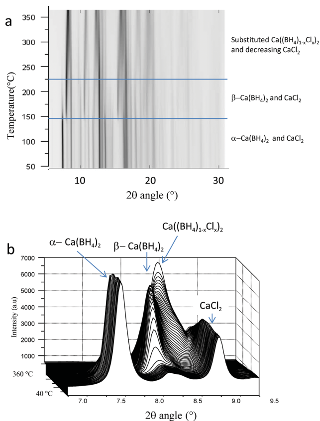
Fig. 1 In situ SR-PXD measured for \text{Ca}(\text{BH}_4)_2 + \text{CaCl}_2 in molar ratio 1 : 1, heating rate 3 \text{ K min}^{-1} . The temperature increases from 40 to 360 \text{ }^\circ\text{C} . (a) gives a plot of the evolution of Bragg peak intensities. (b) 3D plot of selected 2\theta area. \lambda = 0.703511 \text{ \AA} .
