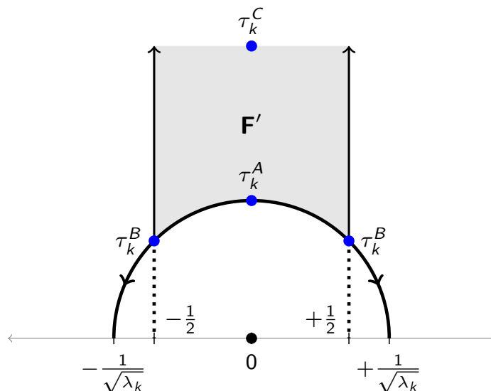
Figure 1. The fundamental domain F' of \Gamma^*(\lambda_k) . The point \tau_k^A is the fixed point of the S , \tau_k^B is the fixed point of ST^{-1} , while \tau_k^C is the fixed point of T .
