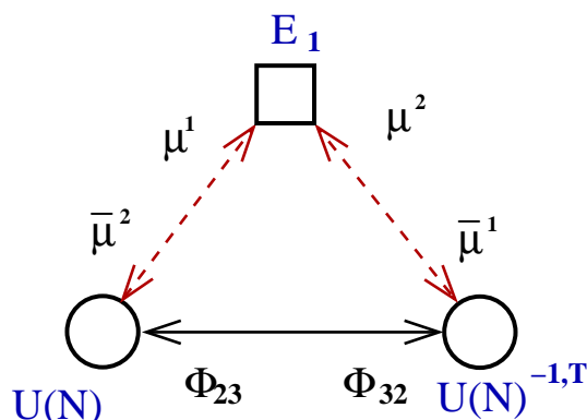
Figure 6: The extended \mathbf{Z}_3 orientifold theory with (0, N) fractional D3-branes and (1, 0) instanton number. The upper node (which would represent the \text{USp}(N_1) gauge group and disappears when we set N_1 = 0 as in the case under consideration) is where the instanton sits. The lower nodes denote only one gauge group. The charged fermionic zero-modes follow eq. (5.11). For simplicity we have not drawn the lines denoting the adjoint.
