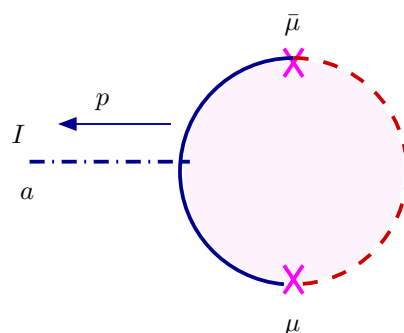
Figure 6: The mixed disk describing the emission of an adjoint scalar \varphi_a^I of momentum p represented by the outgoing dashed line.
