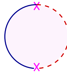
Figure 1: The simplest mixed disk with two-boundary changing operators indicated by the two crosses. The solid line represents the D3 boundary while the dashed line represents the D(-1) boundary.
