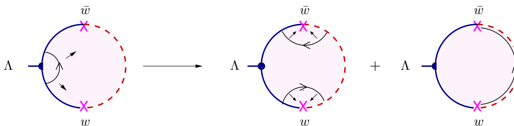
Figure 7: The Ward identity for the broken supersymmetries. The internal oriented line represents the integration contour for the supercurrent M'(j+\tilde{j}) . The diagram in the left hand side corresponds to the term \langle\langle V_{\bar{w}}[M'q', \mathcal{V}_{\bar{\Lambda}^I_{\alpha A}}]V_w \rangle\rangle in (5.20). The two diagrams in the right hand side are obtained by deforming the integration contour. The first of them corresponds to -\langle\langle [M'q', V_{\bar{w}}] \mathcal{V}_{\bar{\Lambda}^I_{\alpha A}} V_w \rangle\rangle - \langle\langle V_{\bar{w}} \mathcal{V}_{\bar{\Lambda}^I_{\alpha A}} [M'q', V_w] \rangle\rangle (where the minus sign is due to the clockwise orientation of the contours), whereas the last diagram corresponds to the right hand side of (5.20).
