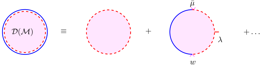
Figure 8: Pictorial representation of the “disk” \mathcal{D}(\mathcal{M}) . For example, the second disk in the r.h.s. corresponds to the amplitude \mathcal{A}_{(w\lambda\bar{\mu})} (see eq. (3.22)) which in the field theory limit gives rise to the term \text{tr}(\bar{i}\bar{\mu}_u^A w_\alpha^u \lambda^{\alpha_A}) of the moduli action.
