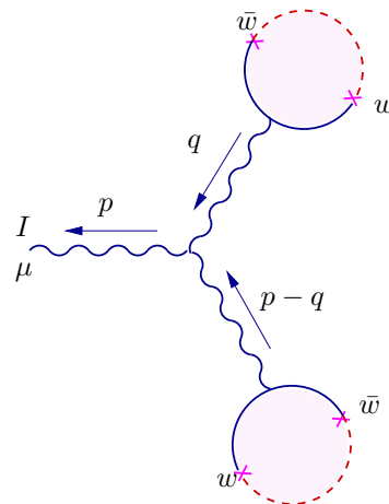
Figure 4: In the field theory limit the mixed disk of figure 3 reduces to this configuration which accounts for the second order term in the large-distance approximation of the instanton solution for the gauge vector.
