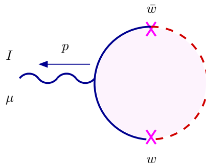
Figure 2: The mixed disk that describes the emission of a gauge vector field A_\mu^I with momentum p represented by the outgoing wavy line.
