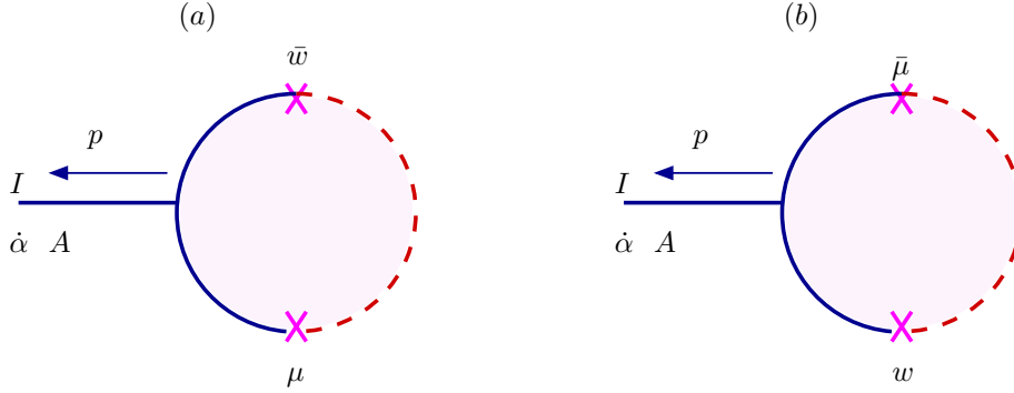
Figure 5: The two mixed disks that contribute to the emission of a gaugino \bar{\Lambda}_{\dot{\alpha}A}^I with momentum p represented by the outgoing solid line.
