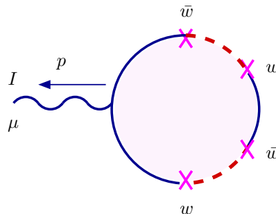
Figure 3: The mixed disk for the second order contribution to the gauge vector.
