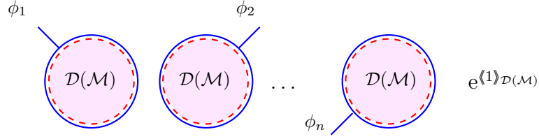
Figure 11: The dominant contribution to an amplitude with n external \mathcal{V}_\phi vertex operators in a D-instanton background is a product of tadpoles.
