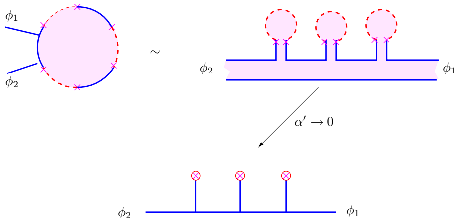
Figure 9: Mixed disk string diagrams correspond in the field-theory limit to interactions of the first-quantized world-lines with the instantonic background.
