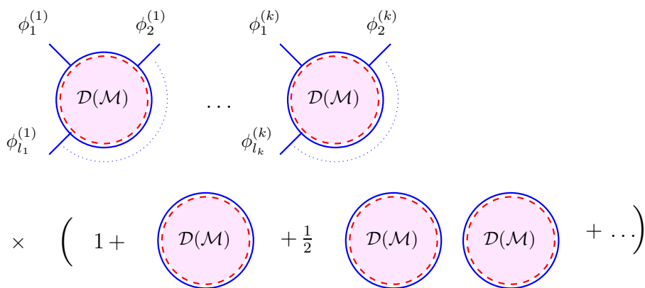
Figure 10: A connected amplitude with n external \mathcal{V}_\phi vertex operators in a D-instanton background receives contributions from topologically disconnected world-sheets, characterized by the insertion of l_i vertex operators for \phi fields in each connected component, with \sum_i l_i = n .
