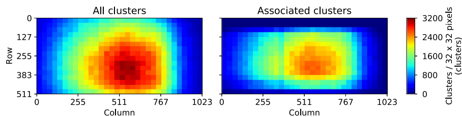
Fig. 6. Distributions of all the clusters on the DUT (left) and of those associated to the tracks (right). Fewer clusters are associated to tracks in columns 376–381 due to exclusion of a dead double column.
