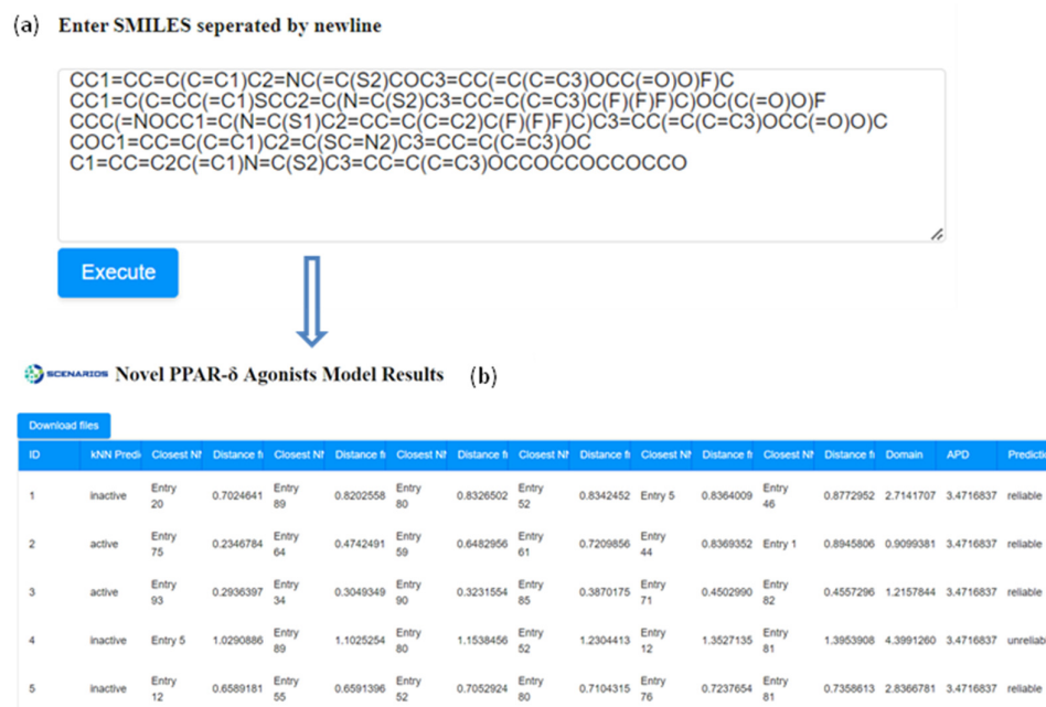
Figure 4. Entering the SMILES notations of five different compounds as input to the web application (a) and the generated output page (b). Out of the five compounds tested, the kNN algorithm identified only the two PFAS congeners (CID 54764927 and 51346913) as active.
