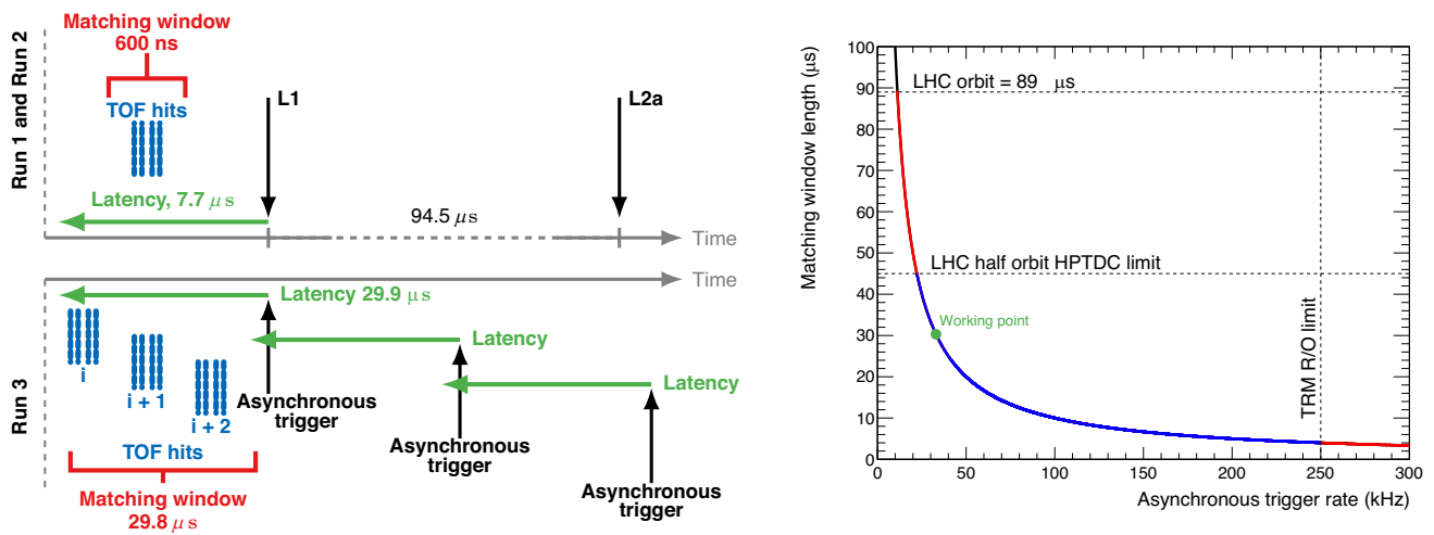
Fig. 2 (left) HPTDC programming schema adopted during Run 1 and 2 (top left) and during Run 3 (bottom left). As described in detail in [7], in Run 3, all triggers used previously are replaced by a periodic trigger (asynchronous with respect to actual collisions) at fixed bunch crossing number ( f = 33.4 kHz), mimicking a continuous readout and covering a complete LHC orbit within three triggers. All hits (short vertical blue lines) are read out and can be associated with physical events at a later stage. (right) Possible selection of parameters (asynchronous trigger frequency f_T and matching window width m_w ) to realize a continuous readout. The blue curve shows the region of allowed values. The red boundaries illustrate system limitations from the HPTDC matching algorithm and HPTDC readout time constraints. The green circle marks the chosen point of operation, with an asynchronous trigger rate of \sim 33 kHz and a matching window of 28.8 \mu\text{s}
