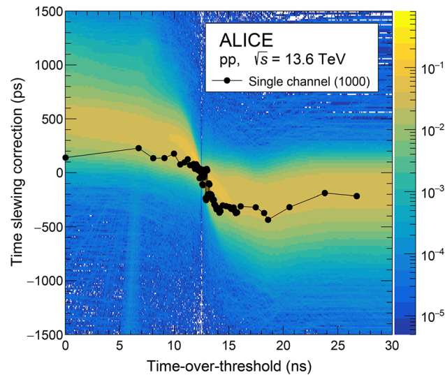
Fig. 4 Distribution of time-slewing corrections: An example for one single channel is provided as a reference superimposed on a color-scale distribution corresponding to the density of all channel-calibration curves. A reference at zero was taken for all channels at ToT = 12.5 ns. The reported time-slewing calibration was obtained from the data taken with pp collisions at \sqrt{s} = 13.6 TeV. Sufficient statistics are required to ensure that the statistical uncertainty on the extracted correction remains below 10 ps. The shape of the correction is driven by the rise-time dependence of the discriminator threshold
