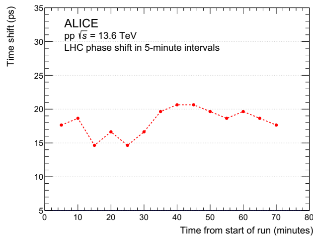
Fig. 3 Example of the TOF clock alignment for a single run extracted in 5-min intervals. The statistical error is significantly smaller than the marker size
