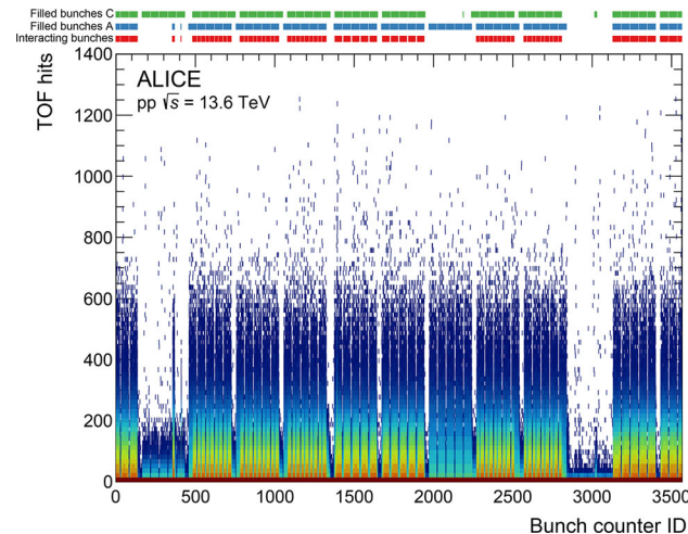
Fig. 5 Hit multiplicity as a function of the bunch counter ID, blue colors represent lower counts. The structure of the LHC filling scheme for the data collected is reported for both beams (A and C) in the top section of the plot, the filling scheme is visible in the TOF hit multiplicity
