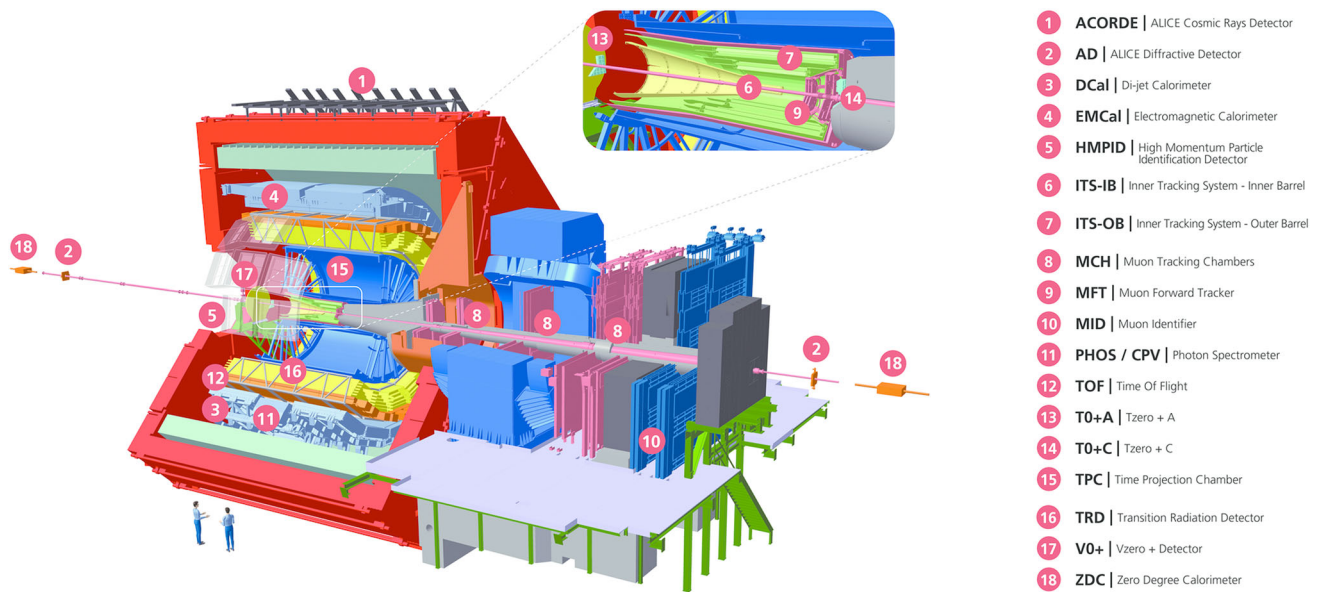
Fig. 1 Schematic of the ALICE detector in Run 3
