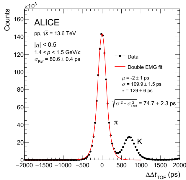
Fig. 9 Distribution of 11t_{\text{TOF}} obtained by considering the track under study in the momentum range 1.4 < p < 1.5 GeV/c. In this momentum range, the peaks corresponding to pions and kaons can be clearly distinguished. The red curve represents the Double EMG fit used to extract the 11t_{\text{TOF}} time resolution. The fit is done over the full range, and the results obtained for different ranges are taken into account in the error
