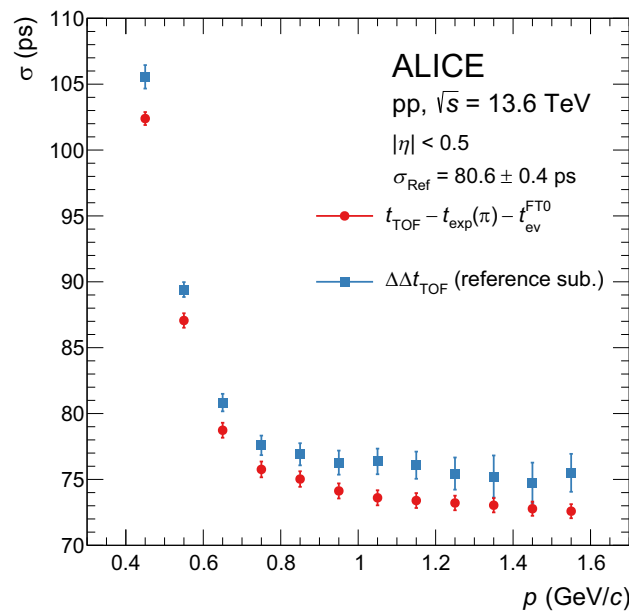
Fig. 11 Timing resolution as a function of momentum p obtained using the 11t_{\text{TOF}} method ( \sigma_{\text{Reference}} is already subtracted) and t_{\text{TOF}} - t_{\text{exp}}(\pi) - t_{\text{ev}}^{\text{FT0}} method. As the tracking momentum resolution improves, with increasing momentum, so does the timing resolution
