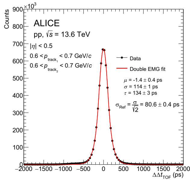
Fig. 7 11t_{\text{TOF}} distribution for the reference tracks, selecting both \text{track}_1 and \text{track}_2 with a momentum in the range 600 < p < 700 MeV/c, represented by the black-shaded band in Fig. 6. The fit is done over the full range of the histogram
