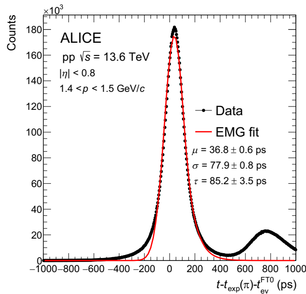
Fig. 10 Distribution of the t_{\text{TOF}} - t_{\text{exp}}(\pi) - t_{\text{ev}}^{\text{FT0}} in the momentum range 1.4 < p < 1.5 GeV/c. The red curve represents the EMG fit used to extract the time resolution. The fit is done in the range (-200, 200) ps, and the results obtained from different ranges are taken into account in the error
