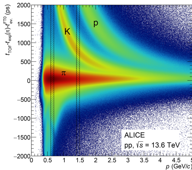
Fig. 6 Time difference measured with TOF with respect to the expected value for the charged-pion mass hypothesis as a function of momentum, blue colors represent lower counts. The two vertical shaded regions indicate momentum ranges used to obtain the final time resolution for the two methods presented in the text
