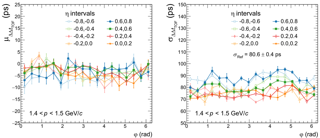
Fig. 12 Distributions of the mean value (left) and sigma (right) using the 11t_{\text{TOF}} method in the momentum range 1.4 < p < 1.5 GeV/c as a function of \phi for different \eta intervals
