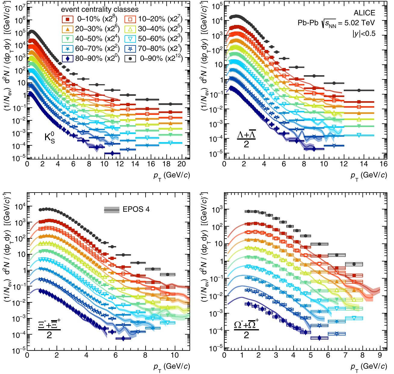
FIG. 3. K_S^0 , \Lambda , \Xi , and \Omega transverse momentum spectra in Pb-Pb collisions at \sqrt{s_{NN}} = 5.02 TeV for different event centrality intervals. Error bars show the statistical uncertainty, while boxes represent the total systematic uncertainty. For each centrality class, predictions from the EPOS4 [36] model are reported as solid lines, with the corresponding transparent area accounting for the statistical uncertainty on the model. Scale factors are applied to both the results and the model to improve visibility.
