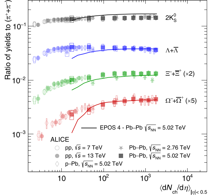
FIG. 5. K_S^0 , \Lambda + \bar{\Lambda} , \Xi^- + \bar{\Xi}^+ , and \Omega^- + \bar{\Omega}^+ particle yield ratios to the pion yield in Pb-Pb collisions at \sqrt{s_{NN}} = 5.02 TeV (squares), compared to results in pp collisions at \sqrt{s} = 7 TeV [28] and \sqrt{s} = 13 TeV [29] (hollow and full circles, respectively), in p -Pb collisions at \sqrt{s} = 5.02 TeV [32] (hollow diamonds), and in Pb-Pb collisions at \sqrt{s_{NN}} = 2.76 TeV [26,59] (stars). Error bars show the statistical uncertainty, while boxes represent the total systematic uncertainty. EPOS4 [36] predictions are reported for the top Pb-Pb energy as solid lines.
