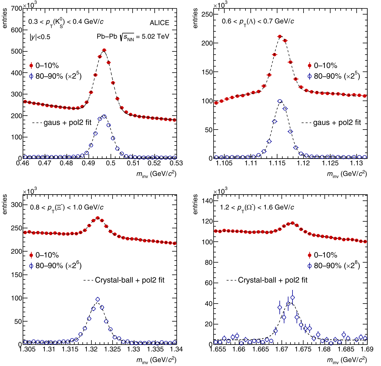
FIG. 1. Invariant mass distributions for (top left) K_S^0 , (top right) \Lambda , (bottom left) \Xi^- , and (bottom right) \Omega^- for the lowest transverse momentum intervals accessed by the analysis. The distributions for the most central (red full markers) and most peripheral (blue open markers) class of events are reported. The dashed lines illustrate the fits used for signal extraction.
