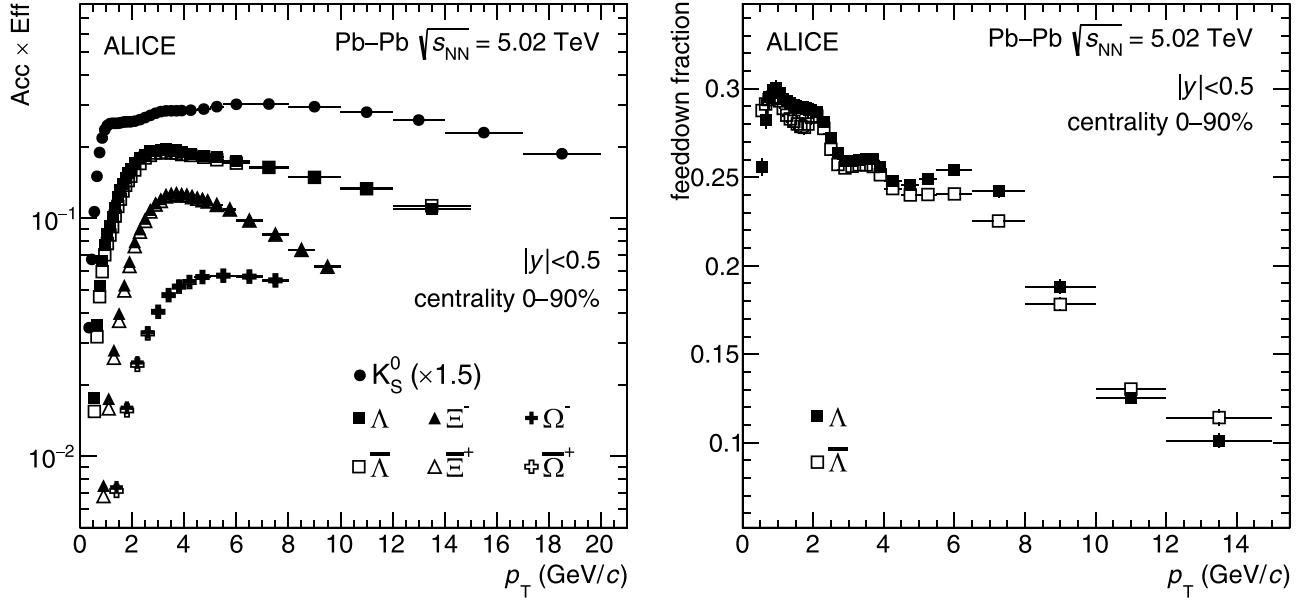
FIG. 2. Left: Acceptance times efficiency ( \text{Acc} \times \text{Eff} ) as a function of p_T for the reconstruction of K_S^0 , \Lambda , \Xi^- , and \Omega^- (full markers) and respective antiparticles (open markers). The 0–90% centrality class is displayed. Right: Ratio of \Lambda coming from charged and neutral \Xi baryon decays to the inclusive \Lambda yield as a function of p_T . Full and hollow markers are for matter and antimatter, respectively. The 0–90% centrality class is displayed.
