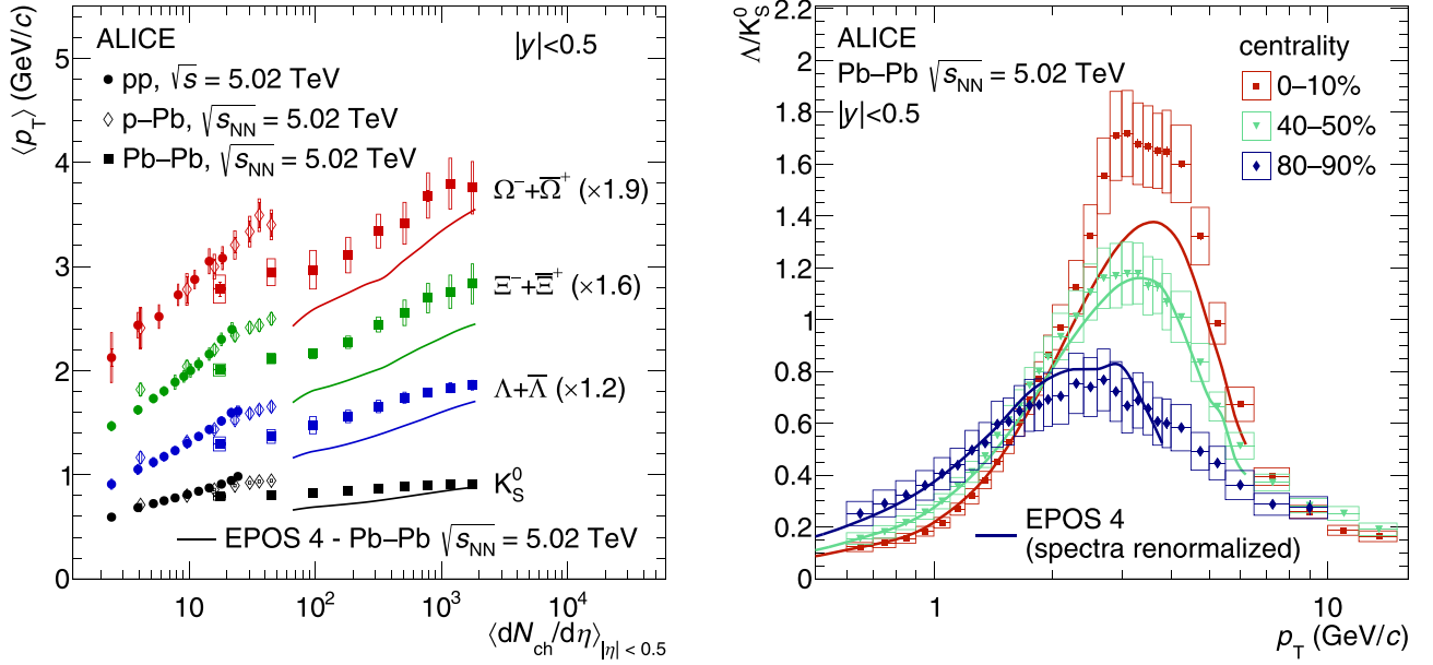
FIG. 4. Left: \langle p_T \rangle as a function of \langle dN_{ch}/d\eta \rangle for K_S^0 , \Lambda , \Xi , and \Omega particle production in Pb-Pb collisions at \sqrt{s_{NN}} = 5.02 TeV at midrapidity (square markers). Results from pp [30] and p-Pb [31,32] collisions at the same center-of-mass energy are also reported as circles and open diamonds, respectively. Error bars correspond to the statistical uncertainty, while boxes correspond to the total systematic uncertainty. Solid lines are predictions from the EPOS4 [36] model. Right: \Lambda/K_S^0 ratio as a function of p_T for the 0–10% most central (red), 40–50% intermediate (green) and 80–90% most peripheral (blue) centrality classes. Error bars correspond to the statistical uncertainty, while boxes correspond to the total systematic uncertainty. EPOS4 [36] predictions, scaled to the total particle yields in the corresponding centrality class, are reported as solid lines.
