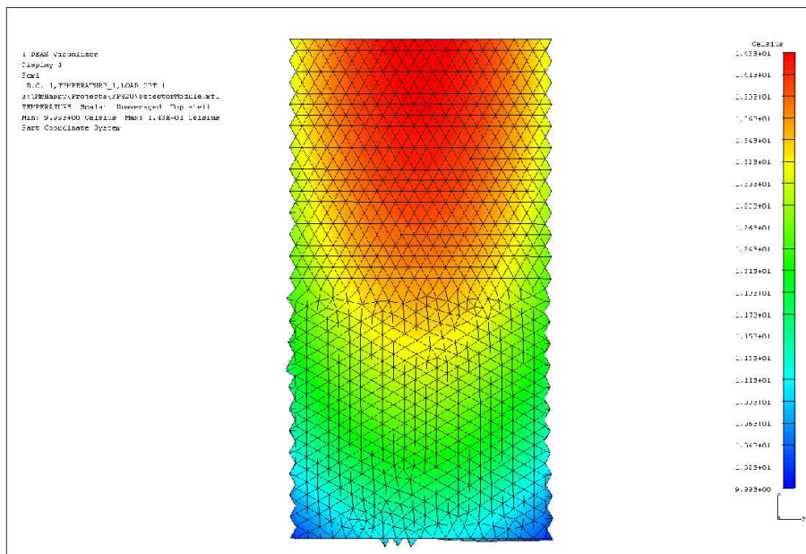
Figure 107. Gradient in the CE7 plane underneath the tracker cell (4.3°C).
