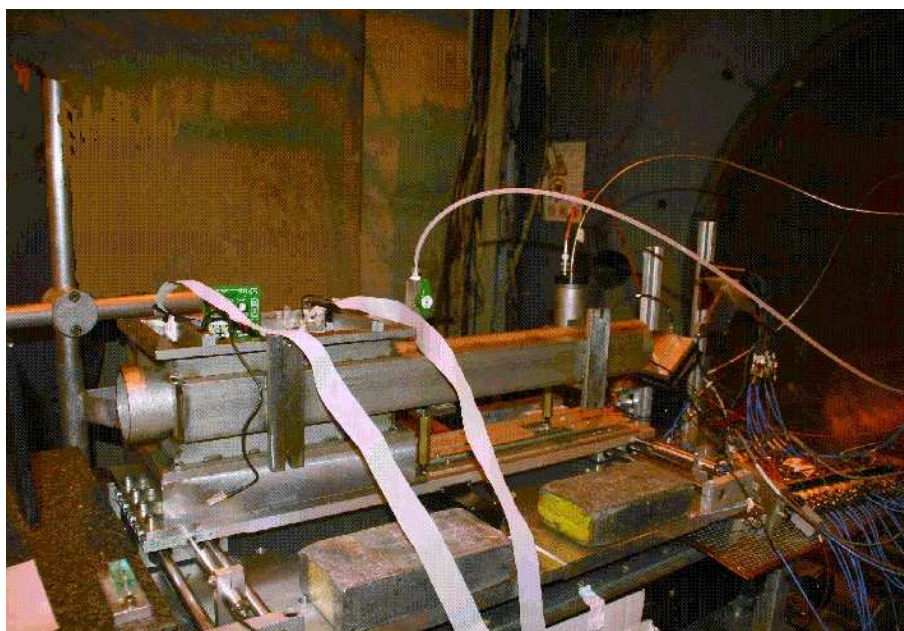
Figure 79. FP420 2007 test beam setup including one movable station, two blades, and two timing detectors (one GASTOF and two QUARTICS).
