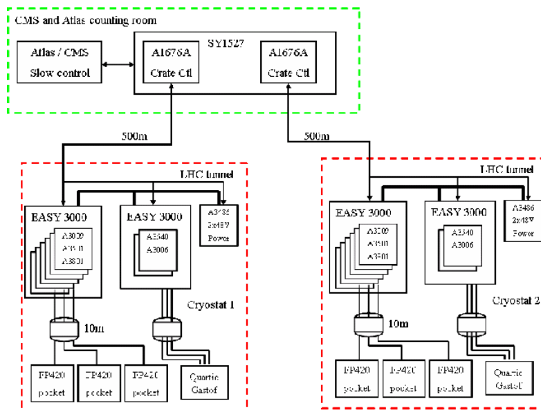
Figure 93. Diagram of the solution suggested by CAEN. The number of pockets assumed is 3 per cryostat. Shown are also the system for temperature monitoring (A3801) and the supplies for QUARTIC/GASTOF detectors (A3540 and A3006).
