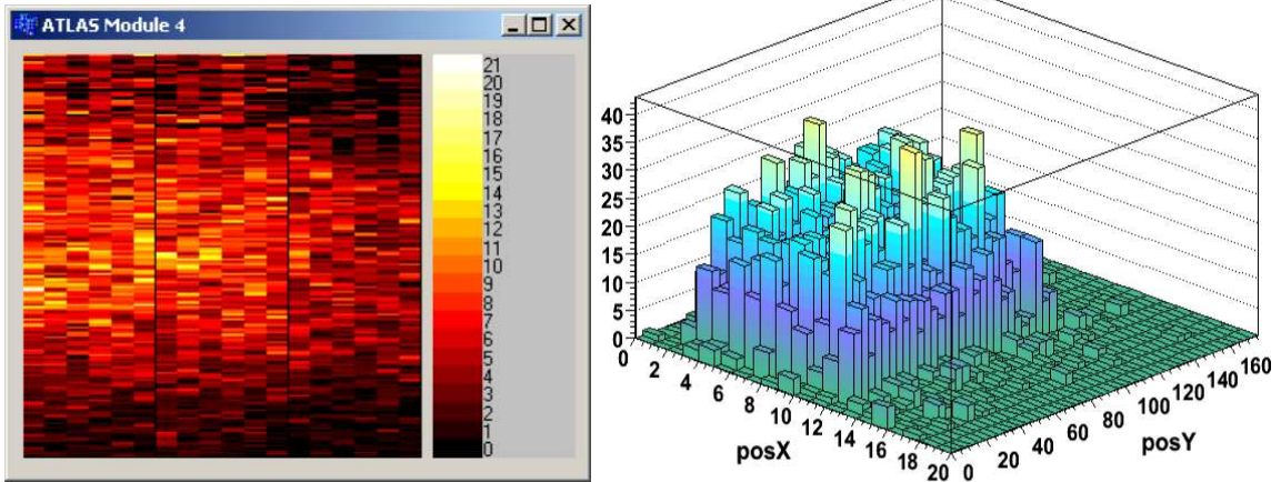
Figure 72. Hit map for a 12 \times 12 \text{ mm}^2 (left) and lego-plot for a 3 \times 3 \text{ mm}^2 (right) scintillator trigger. Device 3D-2E-A operated at 30 V.
