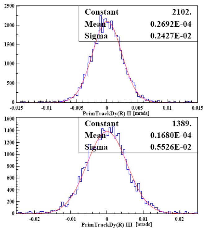
Figure 110. GEANT4 estimate of the multiple scattering (in mrads) in the middle (top) and at the end (bottom) of the three-station tracker.
