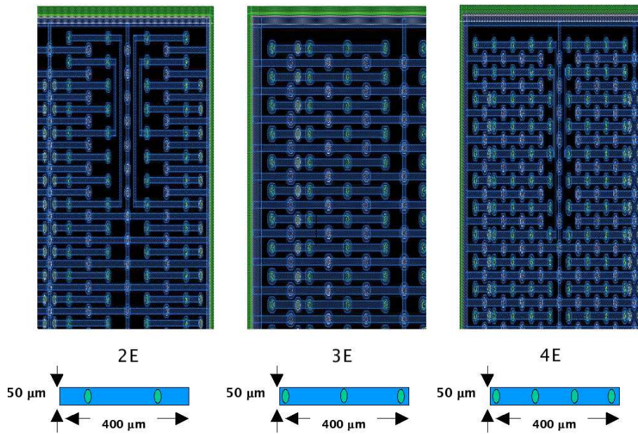
Figure 69. Different 3D cell structures designed to be compatible with the ATLAS Pixel detector readout chip. The pixel size is 50 \mu\text{m} by 400 \mu\text{m} . The devices have either 2, 3 or 4 electrodes per pixel and are named 2E, 3E and 4E respectively. The electrodes cover 4%, 6% and 8% of the total area for 2E, 3E and 4E devices respectively.
