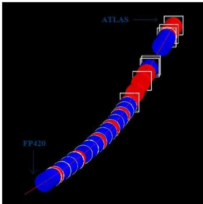
Figure 41. Beam line model created with BDSIM, showing the beamline from ATLAS to the position of the FP420 detector (red denotes a quadrupole element and blue donates a bending element).
