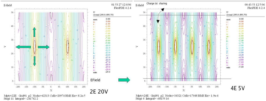
Figure 70. Equipotentials in a 2E and 4E 3D detector. Pixel size is 50 \mu\text{m} (Y) by 400 \mu\text{m} (X). The bias is 20 V and 5 V for the 2E and 4E devices respectively. The direction of the electric field is indicated. The n-electrodes are at the centre. A maximum field of 1 \text{ V}/\mu\text{m} occurs at 24 V and 14 V in a 2E and 4E device respectively.
