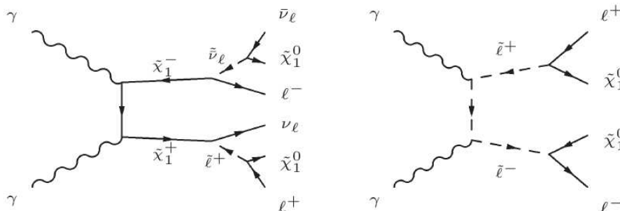
Figure 10. Relevant Feynman diagrams for SUSY pair production with leptons in the final state: chargino disintegration in a charged/neutral scalar and a neutral/charged fermion (left); slepton disintegration (right) [12].
