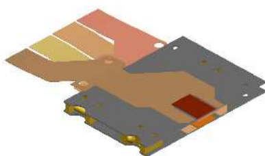
5. Blades A&amp;B assembled to form a superplane
