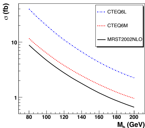
Figure 2. The cross section for the central exclusive production of a Standard Model Higgs boson as a function of M_h , for three different proton parton distribution functions.
