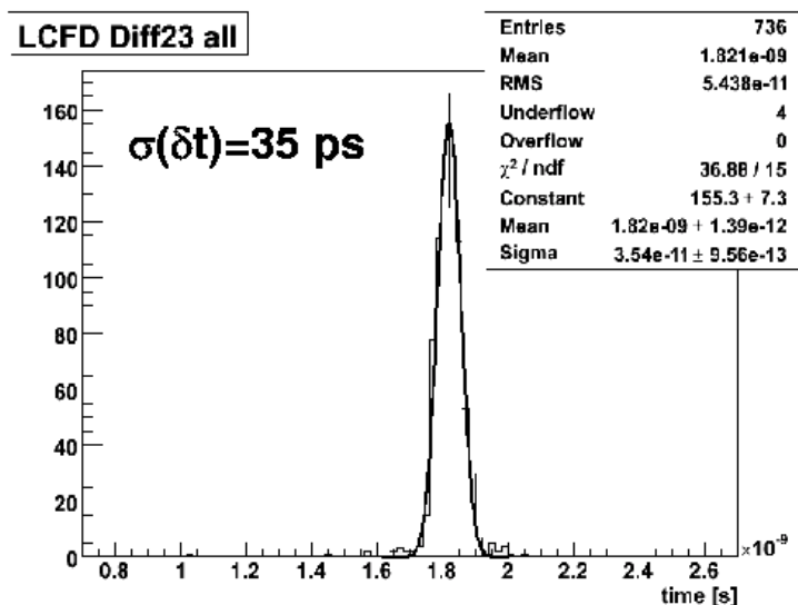
Figure 117. The time difference between the first (G1) and second generation (G2) GASTOF prototype detectors from the March 2007 test beam.
