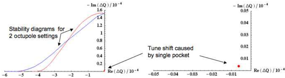
Figure 64. Tune shift induced by FP420 single pocket at 3 mm, due to resistive wall transverse impedance (calculations based on B. Zotter and E. Metral’s models). The effect is negligible when compared to the stability diagram that assesses how the LHC octupoles tuning can damp the instability.
