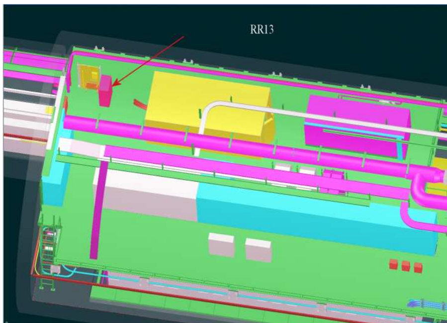
Figure 127. Reserved rack space in the LHC alcove areas (RRs).
