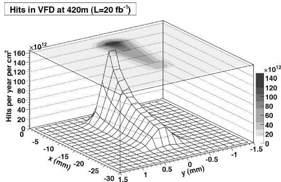
Figure 30. Number of proton hits due to the process pp \rightarrow pX for 20 \text{ fb}^{-1} integrated luminosity. Protons were generated with PYTHIA 6.2.10 (single diffraction process 93) and tracked through the beam lattice with HECTOR.
