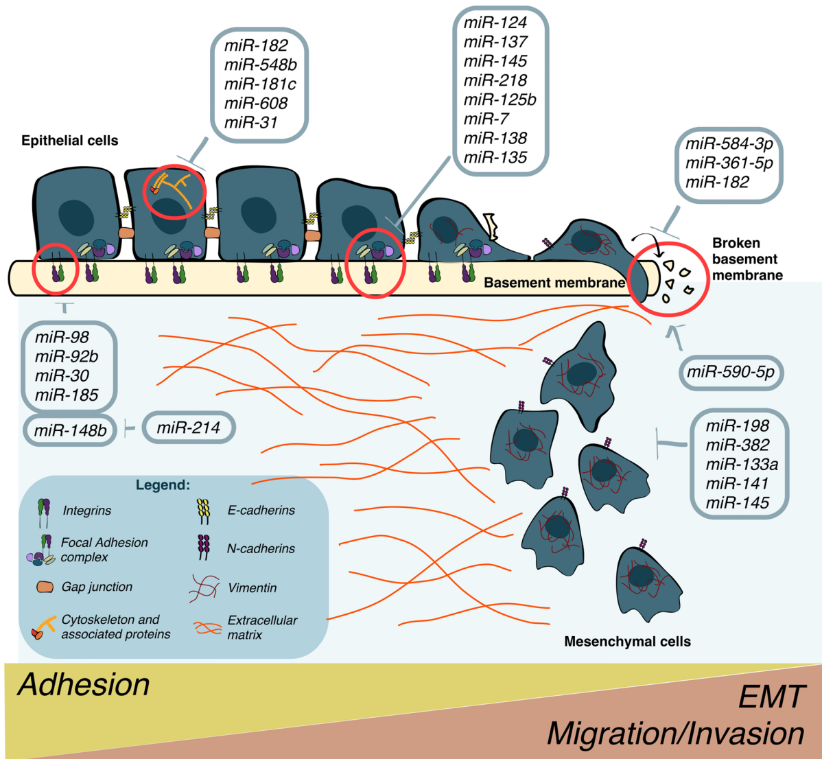
Fig. 3 The adhesome is affected by miRNAs. The figure shows the miRNA-dependent post-transcriptional regulation of gene expression involved in adhesion and epithelial to mesenchymal transition (EMT)
