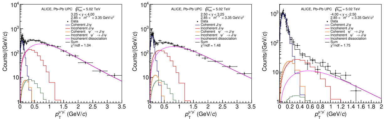
FIG. 4. Transverse momentum distribution of the dimuons for the three rapidity intervals studied with the muon spectrometer.
