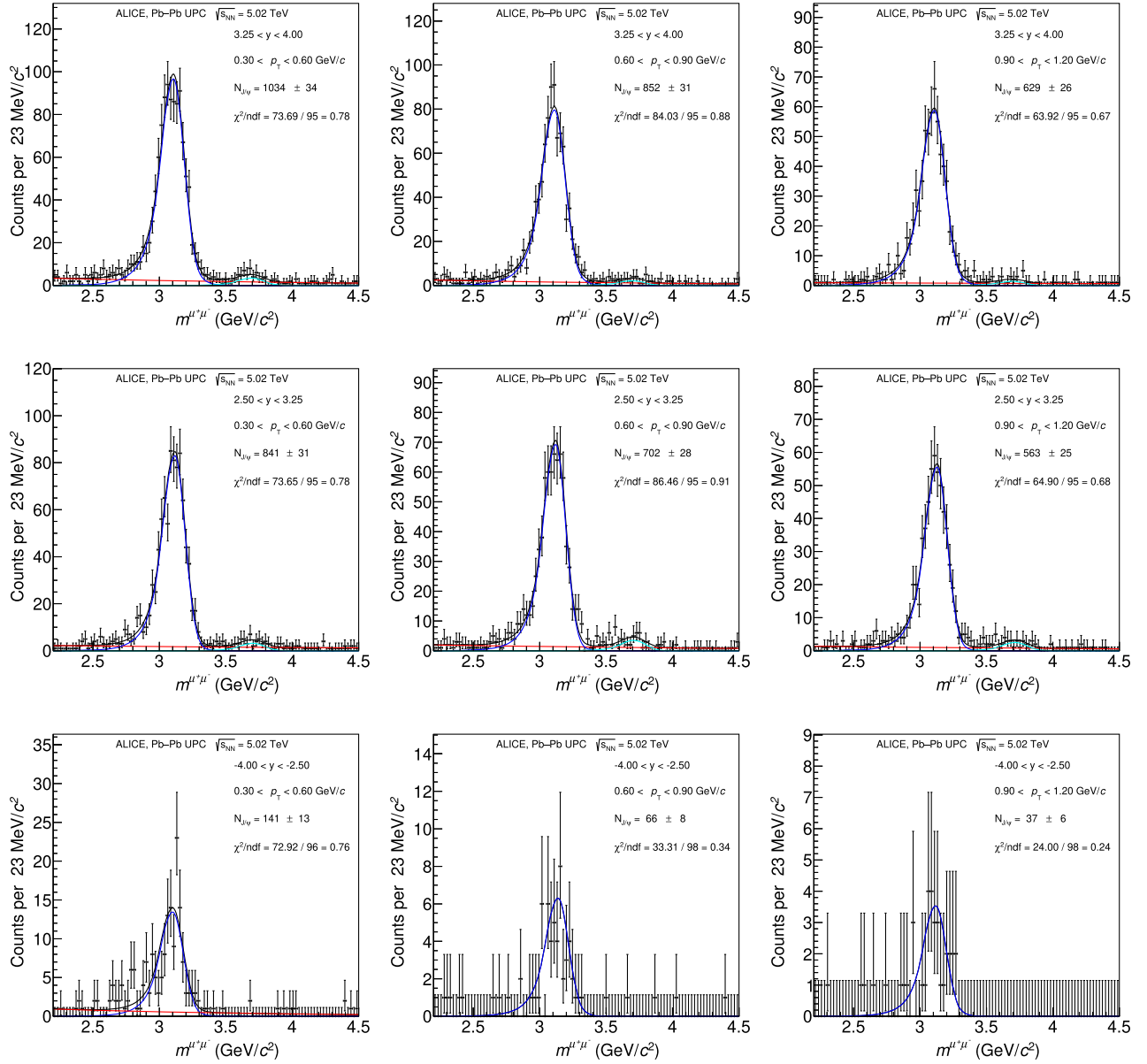
FIG. 3. Dimuon invariant mass distributions in p_T and y intervals and the corresponding extended unbinned likelihood fits. The value of \chi^2 , which is not defined for unbinned fits, is provided for illustration purposes only and correspond to the chosen binning scheme of this figure.
