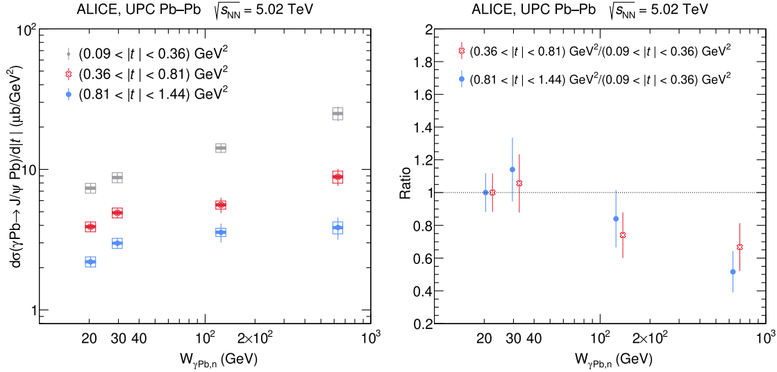
FIG. 1. The energy dependence of the cross section of incoherent J/\psi photonuclear production off lead nuclei is shown for three different ranges of the Mandelstam- t variable (left). The symbols denote the measured cross section, the vertical lines across them represent the uncorrelated uncertainty, the open boxes the correlated uncertainty, and the horizontal shadow box the uncertainty from the computation of the photon flux. Ratio of the cross sections at different Mandelstam- t ranges (right) normalized such that the lower energy ratio is one. The vertical line denotes the statistical and |t| -uncorrelated systematic uncertainties added in quadrature. In the left panel the data symbols have been slightly displaced horizontally to improve their visibility.
