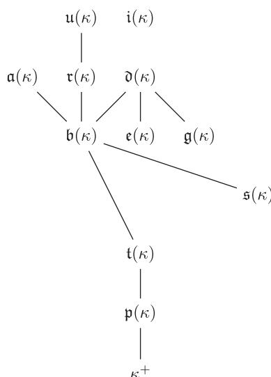
Fig. 3 Diagram of the generalised combinatorial cardinal characteristics (for a fixed \kappa ).
