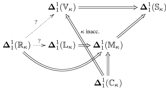
Fig. 4 Diagram of implications for \mathbb{P} -measurability of \Delta_1^1 sets.
