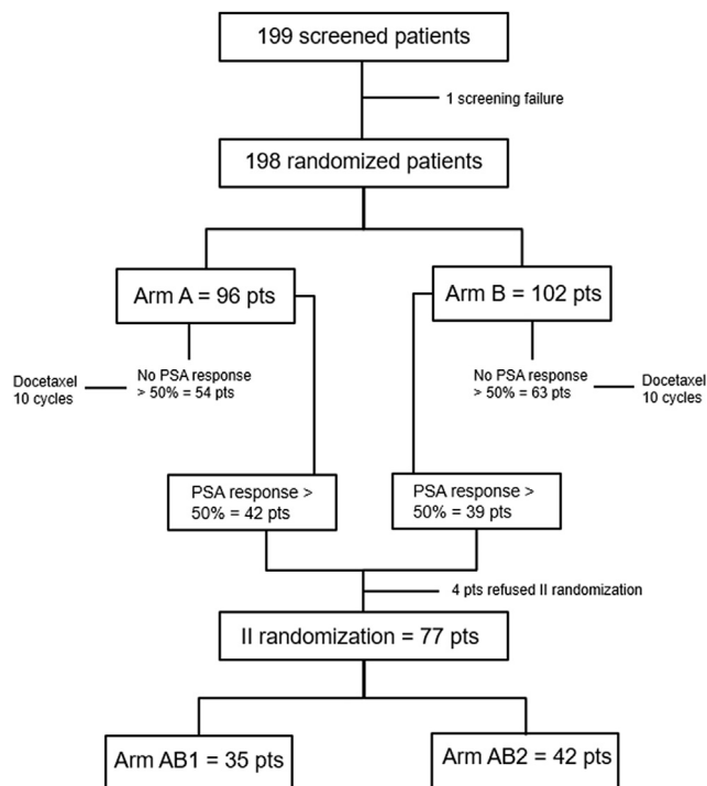
Fig. 1. Consort diagram.
